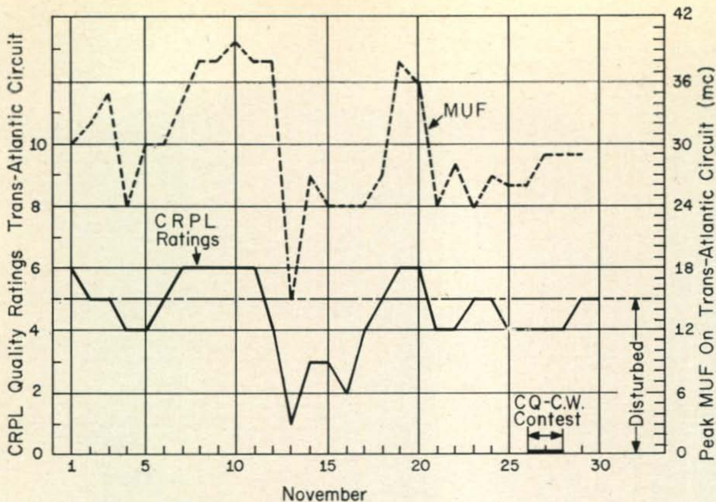
Fig. 1—Daily propagation conditions during November, 1960 and peak MUF's observed on Trans-Atlantic circuits.
