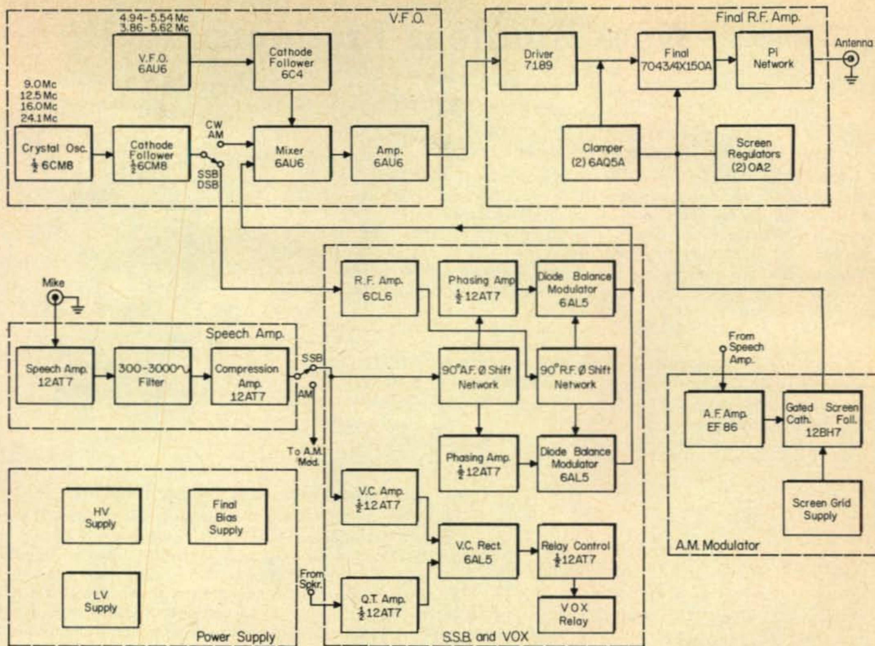
Fig. 1—Block diagram of the new Knight T-400 transmitter with all accessory units. The basic v.f.o., exciter, final amplifier and power supply are standard, while accessory a.m., s.s.b., scope and speech amplifier units are also available.
