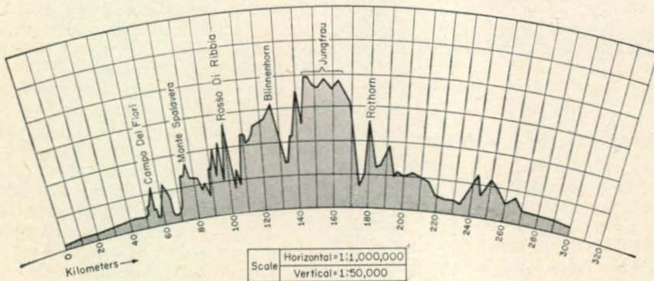
Mario, I1ER, sent along this profile of a path between I1ER and F3AR. Scale, horizontally, is 1:1'000. Vertically, 1:50.
