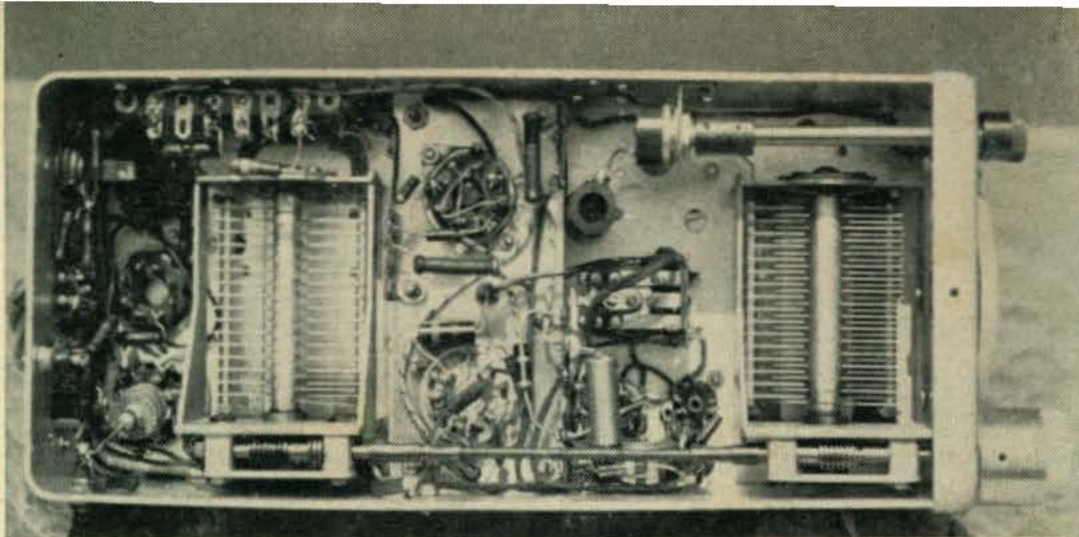
Under-chassis view of the converted BC-458. Only three plates remain in the variable capacitor at the left. The variable capacitor on the right is not used except to mount the v.f.o. dial mechanism. Key jack, power plug and auxiliary contacts for receiver muting are mounted on the rear apron. The 12AX7 and 0A2 regulator are mounted below the relay. Switch S_2 is controlled by the knob at the upper right.
