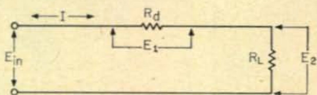
Fig. 4—An equivalent circuit showing that when the diode resistance is low, and the load resistance high, the voltage across R_d is small
