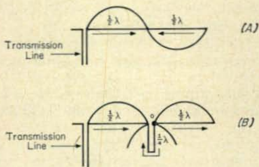
Fig. 4—Phase relationships between two adjacent half wave elements. By use of stubs, phase relationship can be adjusted.
