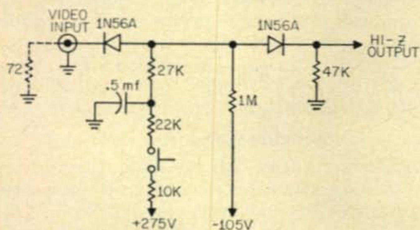
Fig. 2—Two back-to-back diodes will reduce the feedthrough capacity.
