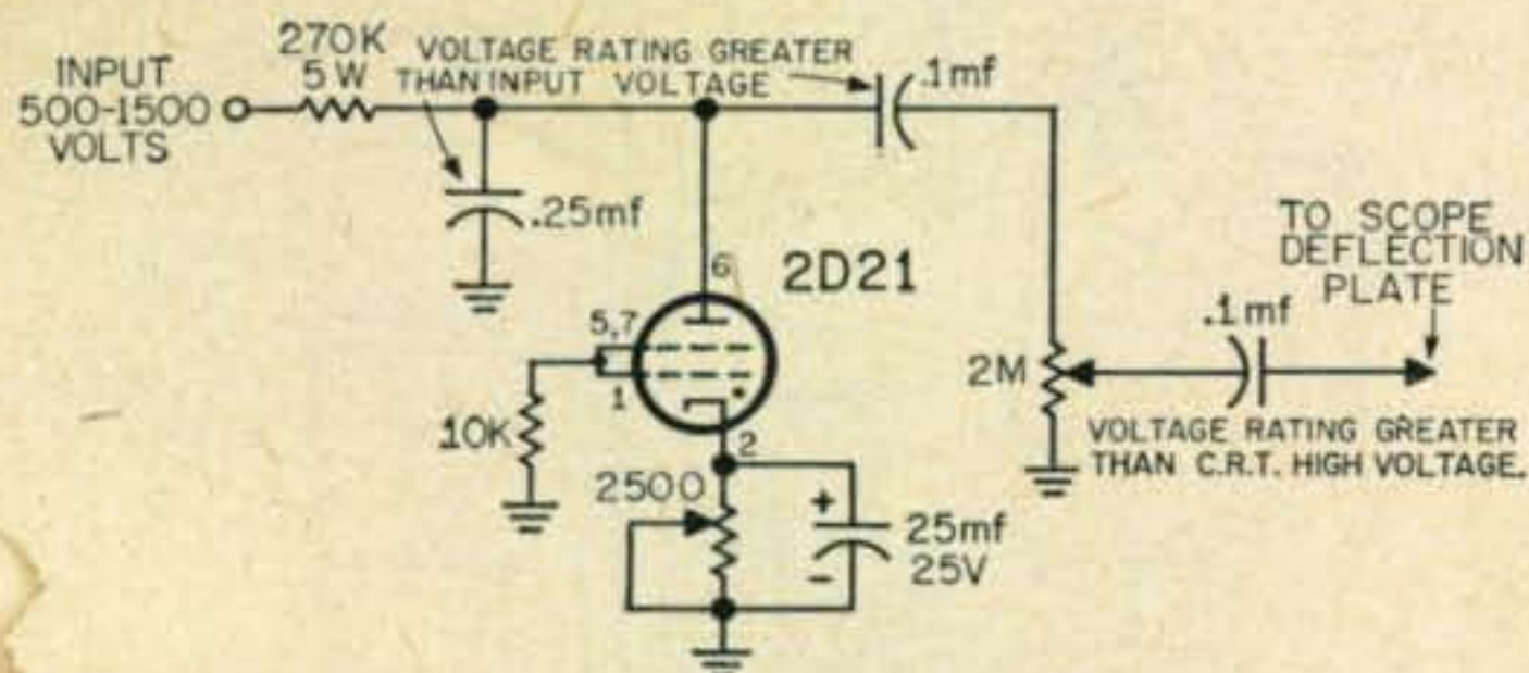
Fig. 1—A thirty cycle thyratron sawtooth generator circuit.
