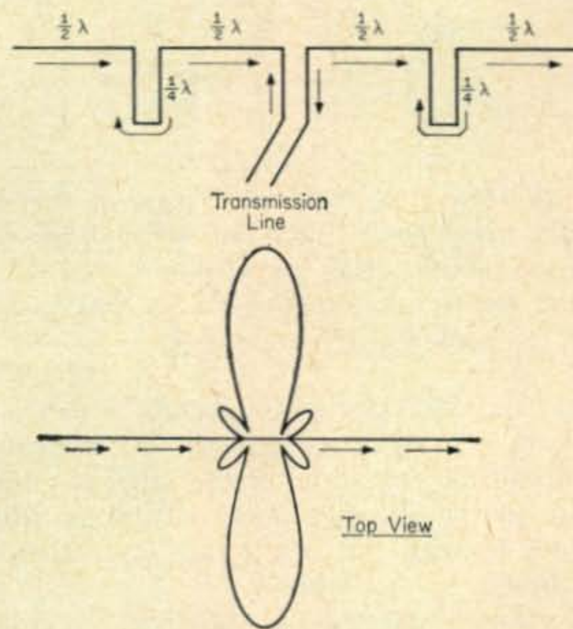
Fig. 5—Four stub-connected collinear elements and the radiation pattern they produce.
