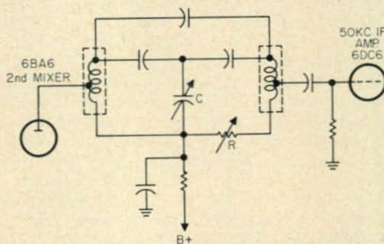
Fig. 2—Equivalent circuit of the i.f. coupling system used in the SX-111 circuit Q is controlled by resistor R.
