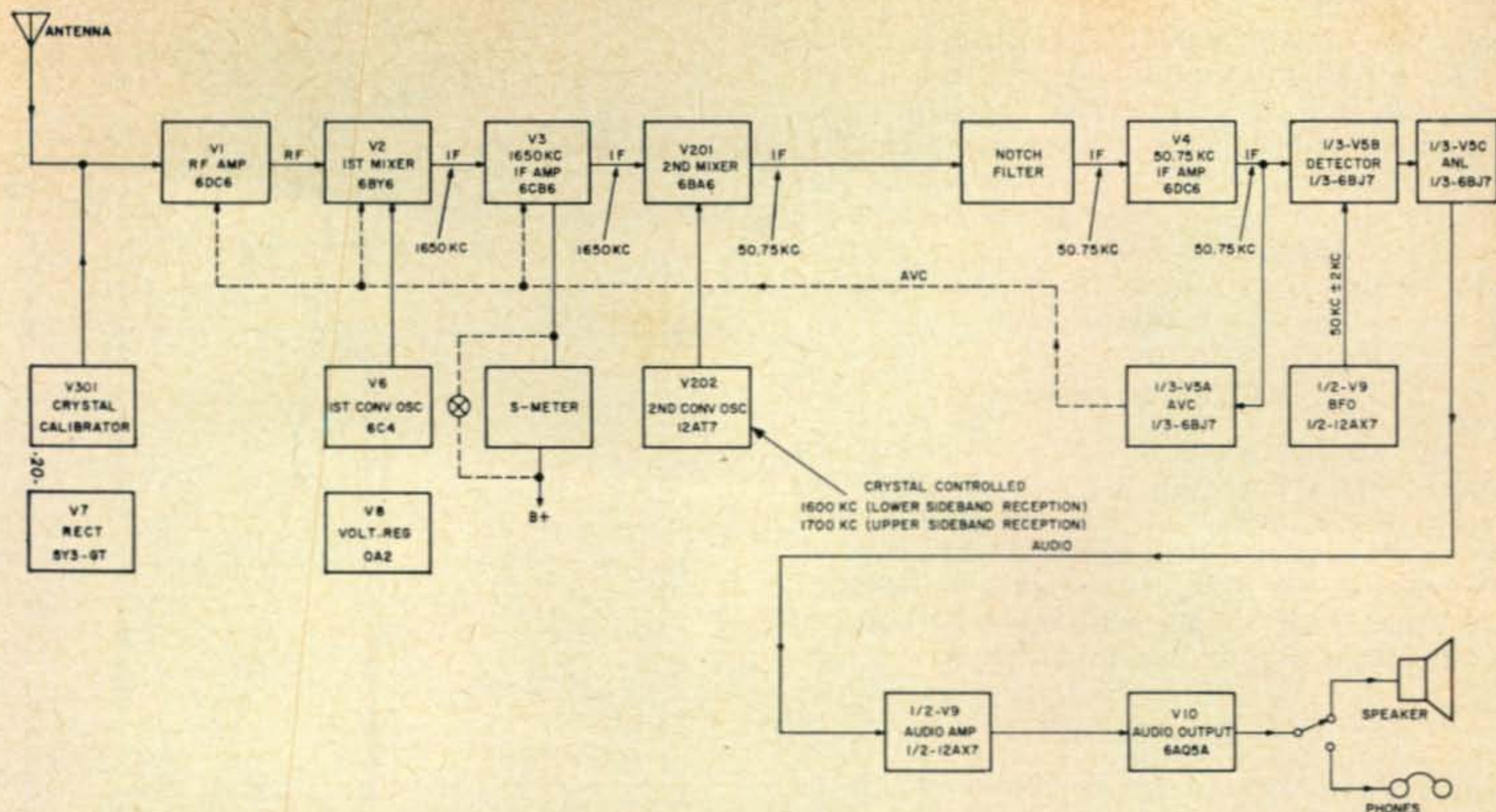
Fig. 1—Block diagram of the new SX-111 receiver. The newer SX-111 Mark I incorporates a product detector located between V 4 and V 5 in the block diagram.
