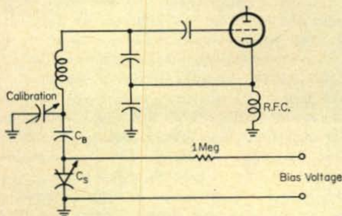
Fig. 3—The Clapp oscillator modified for use with a voltage variable silicon capacitor for remote d.c. tuning.
