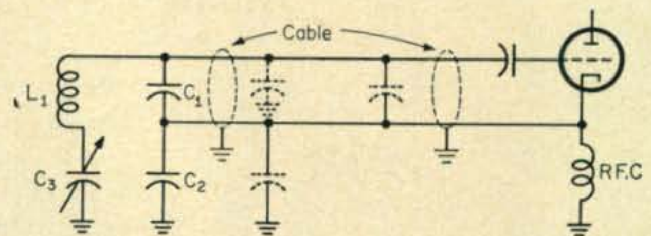
Fig. 2—Schematic representation of the miscellaneous capacitors introduced by the addition of RG-22/U Twinax for remote control of the Clapp oscillator.
