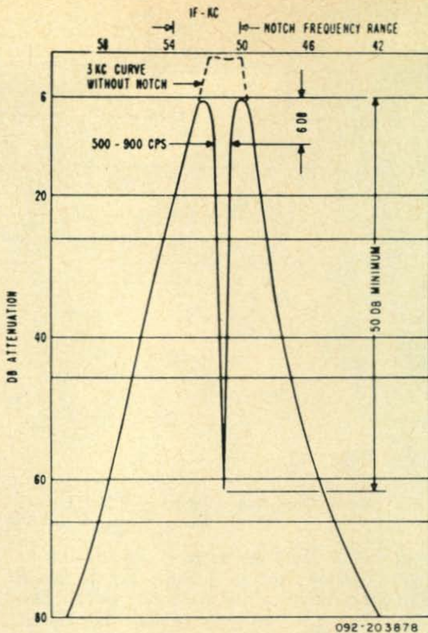
Fig. 5—Graph illustrating notch frequency and depth with relation to the 3 kc selectivity curve.
