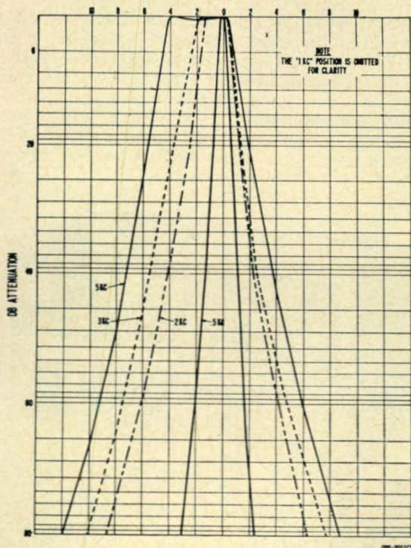
Fig. 3—Diagram illustrating the selectivity of the SX-111 in the various positions of the selectivity switch. Note that the "1 kc" position is eliminated for clarity.
