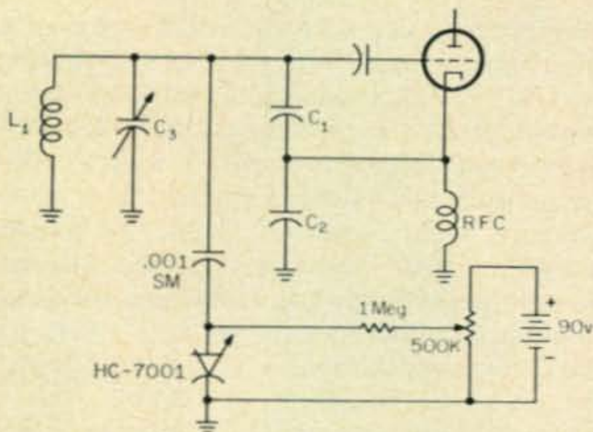
Fig. 5—Silicon capacitor control circuit applied to the parallel tuned Colpitts oscillator
