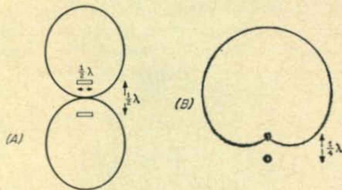
Fig. 7—End-fire array patterns. Figure (a) shows the bidirectional pattern obtained with half wave spacing and feeding 180^\circ out of phase. With 90^\circ feed and quarter wave spacing the unidirectional pattern of (b) is obtained.
