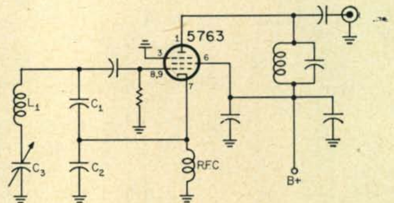
Fig. 1—Diagram of the conventional Clapp oscillator circuit commonly used in amateur applications.
