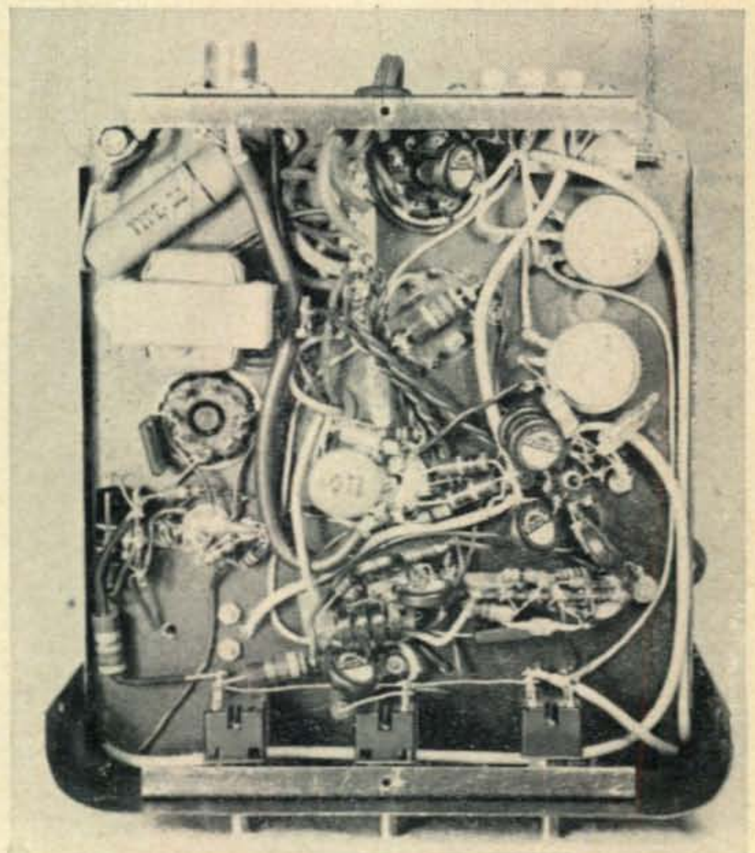
Bottom view. Transformer T_2 is in the upper left corner. One NE2 is located above the 1V2 socket (center) and the other NE2 above the 12AX7 socket on the left (below R_3 ).
