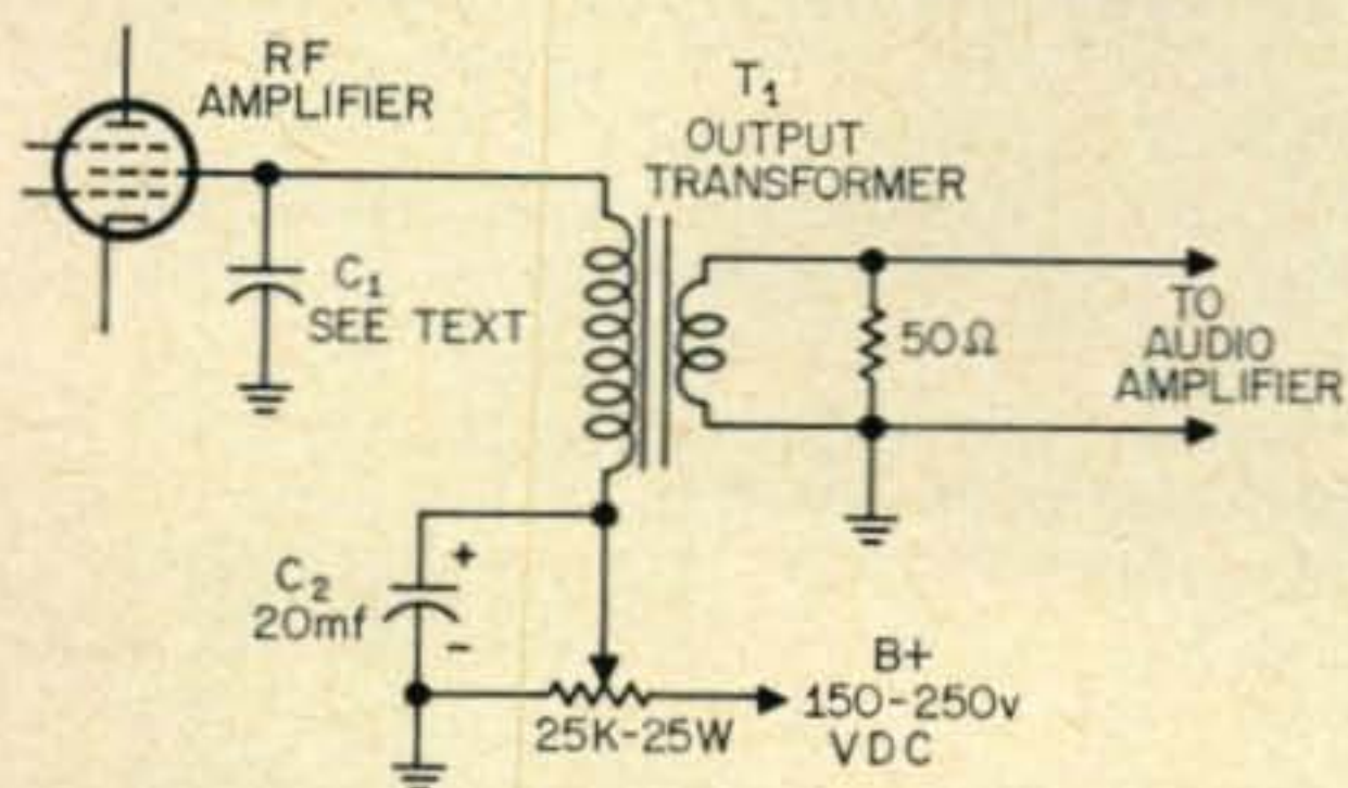
Fig. 1—Diagram of the screen grid modulator. T 1 is a small audio output transformer, primary 5000-10,000 ohms, secondary, 4-8 ohms Stancor No. A3879.
