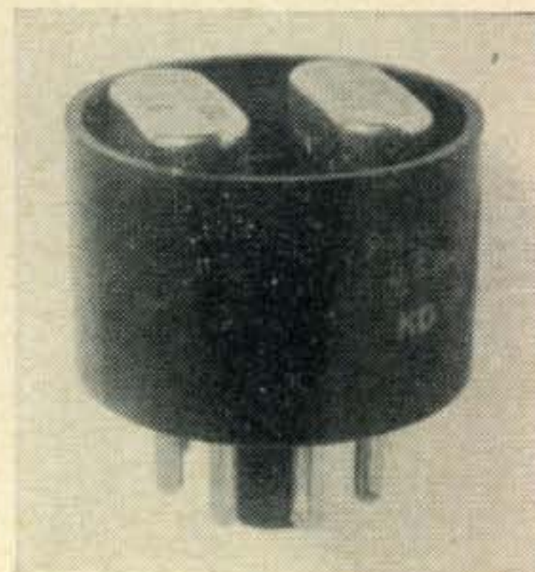
Pair mounting of hermetically sealed crystals to fit standard octal sockets.
