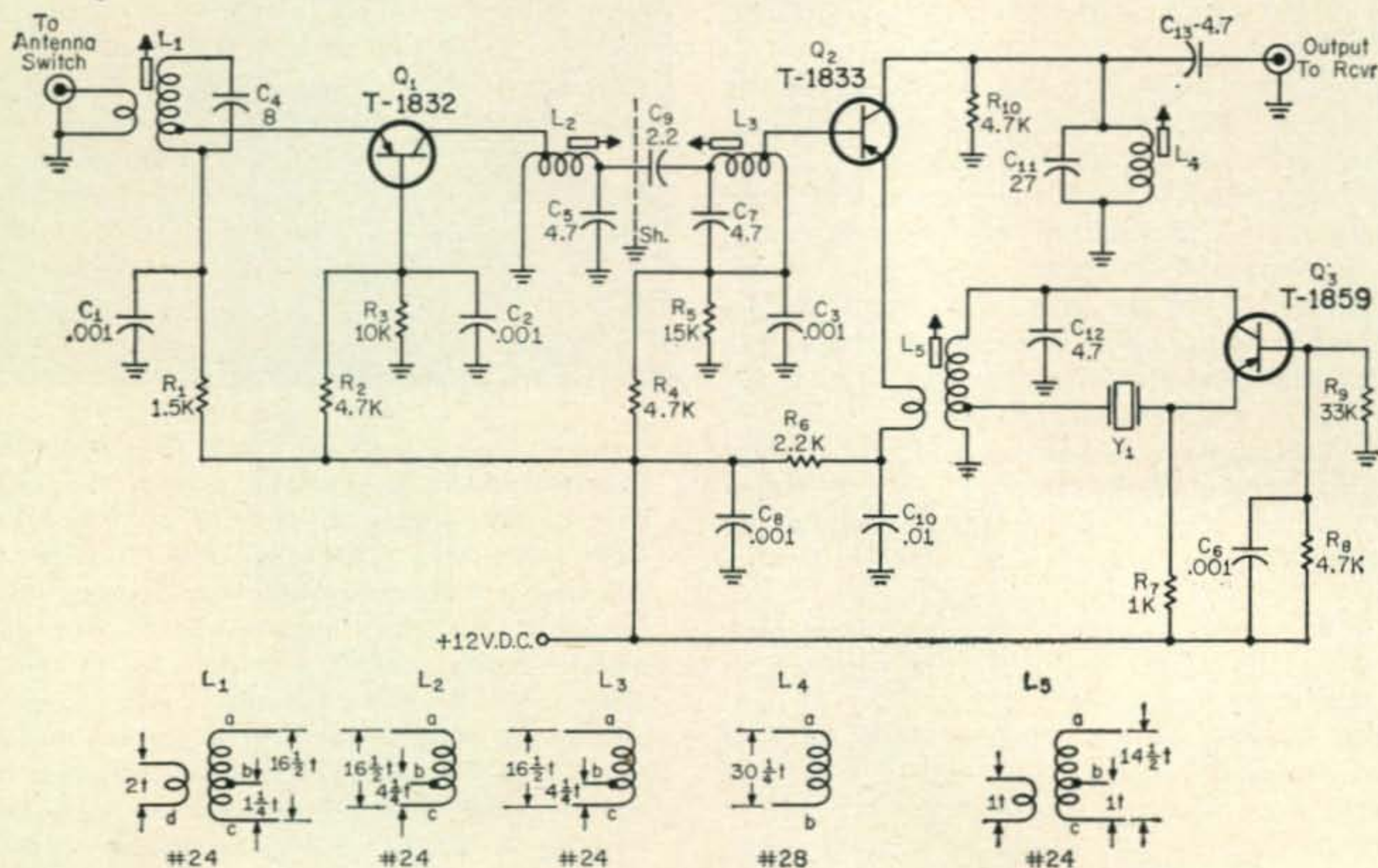
Fig. 1—Six meter converter schematic.
