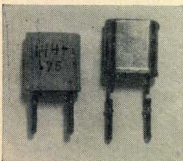
Modifying small pin crystal holders for use in standard crystal sockets.
