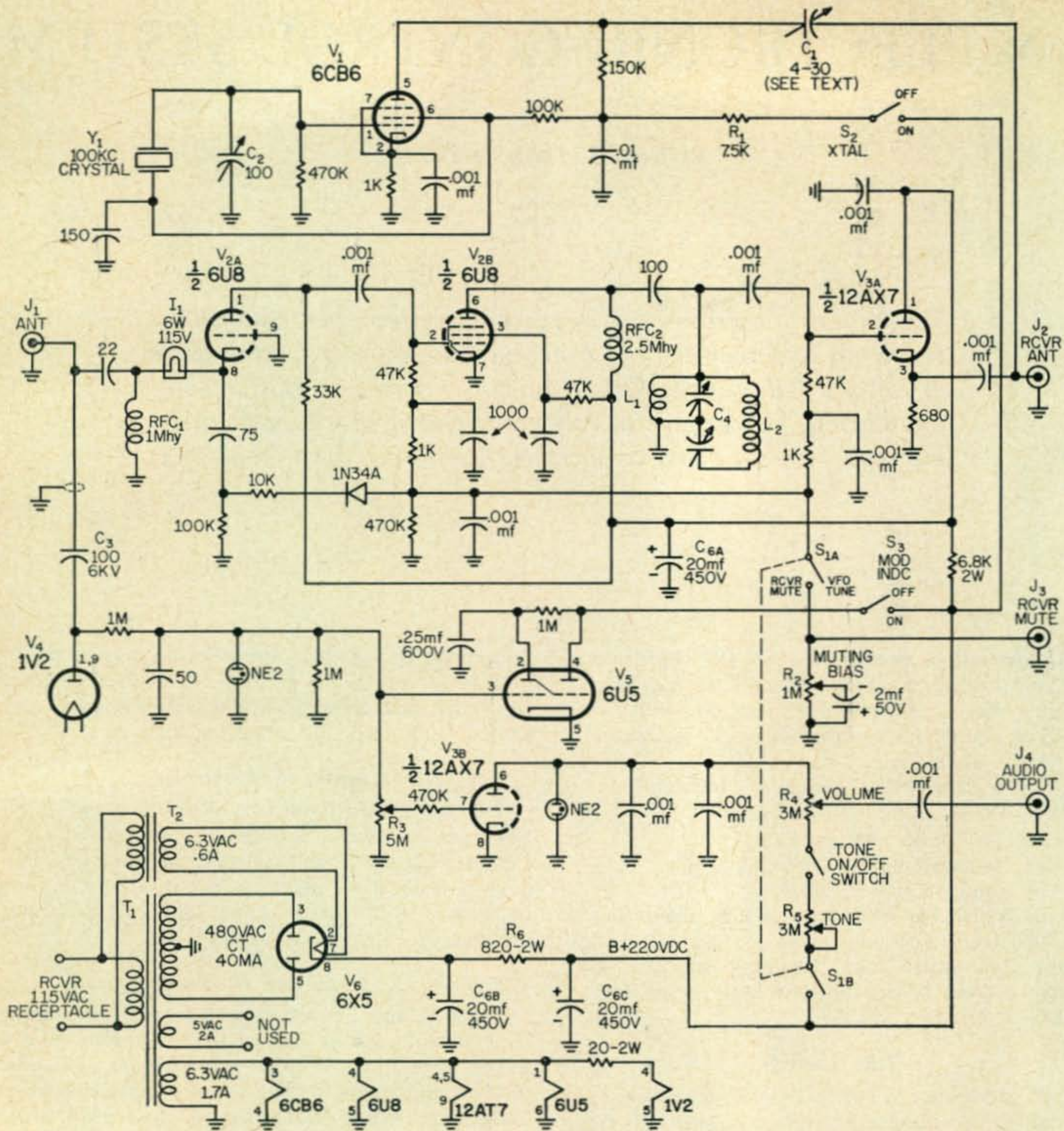
Fig. 1—Schematic of an "Electronic Control System" which includes a 100 kc crystal calibrator, T-R switch, modulation indicator, receiver muting, c.w. audio tone oscillator and a common power supply. All resistors are 1/2 watt and all capacitors are disc ceramic unless otherwise specified.
