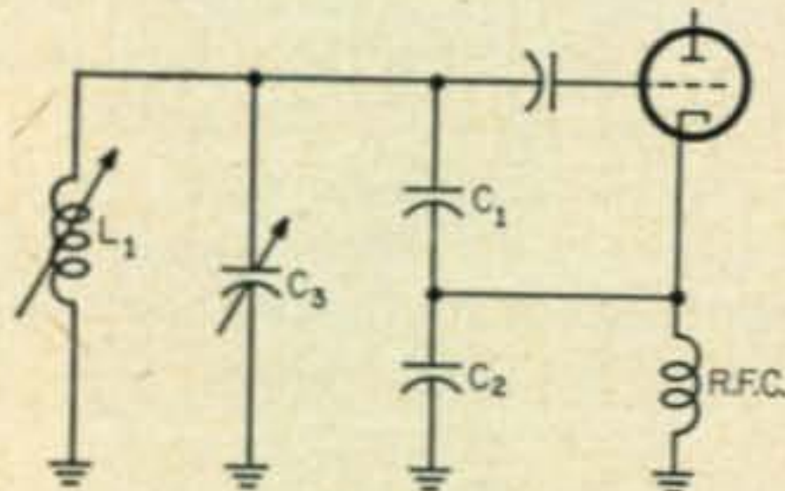
Fig. 4—The high C parallel tuned Colpitts oscillator suitable for remote tuning by use of a voltage variable silicon capacitor.
