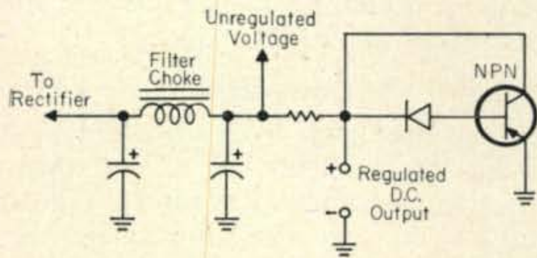
Fig. 1—One method of regulating low d.c. voltages at low currents using a transistor and a reverse connected diode.
