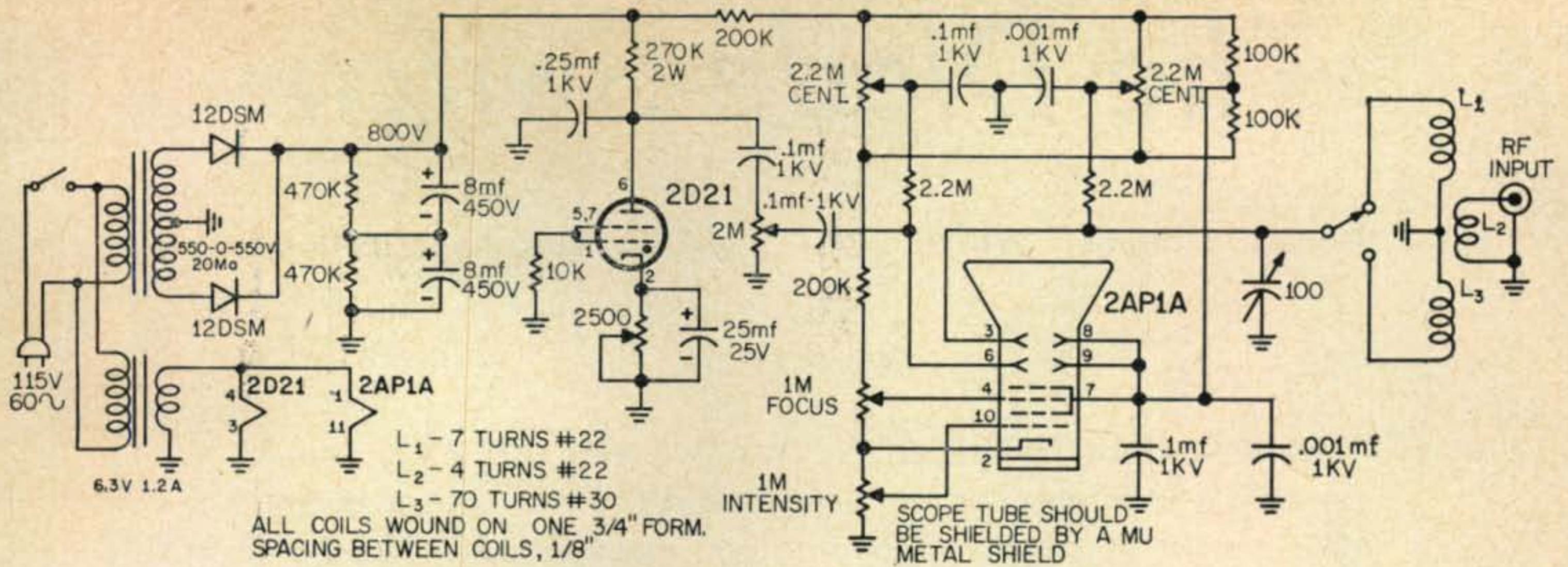
Fig. 2—An a.m. s.s.b. modulation monitor employing the thyatron sweep circuit.
