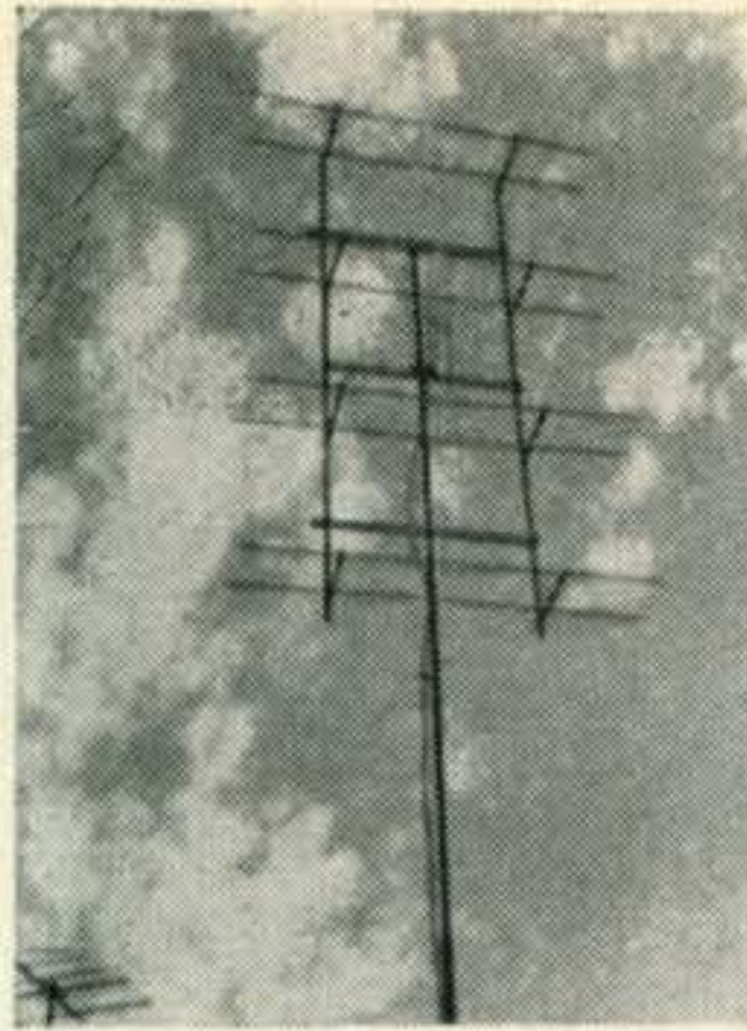
16 element phased array for 432 mc at LU9AT.
