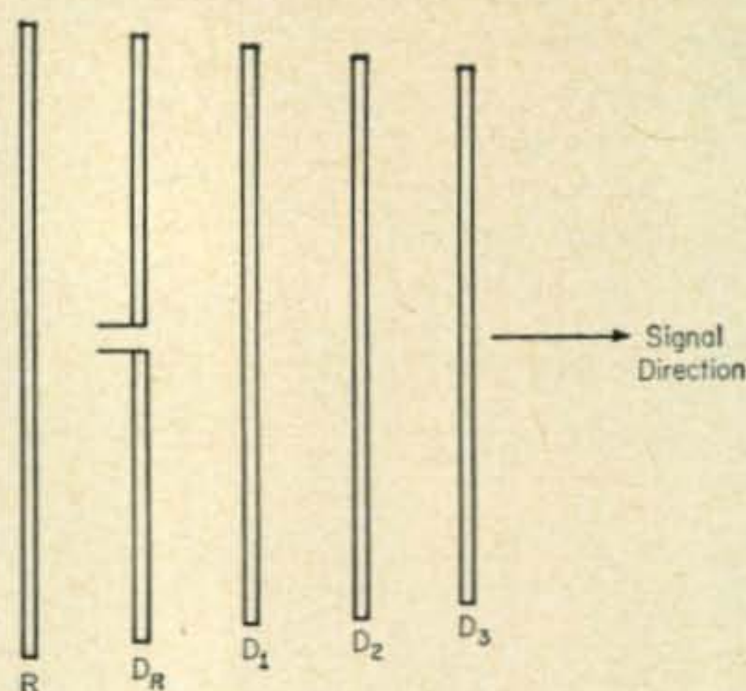
Fig. 3—One type of Yagi array having a reflector and three directors.
