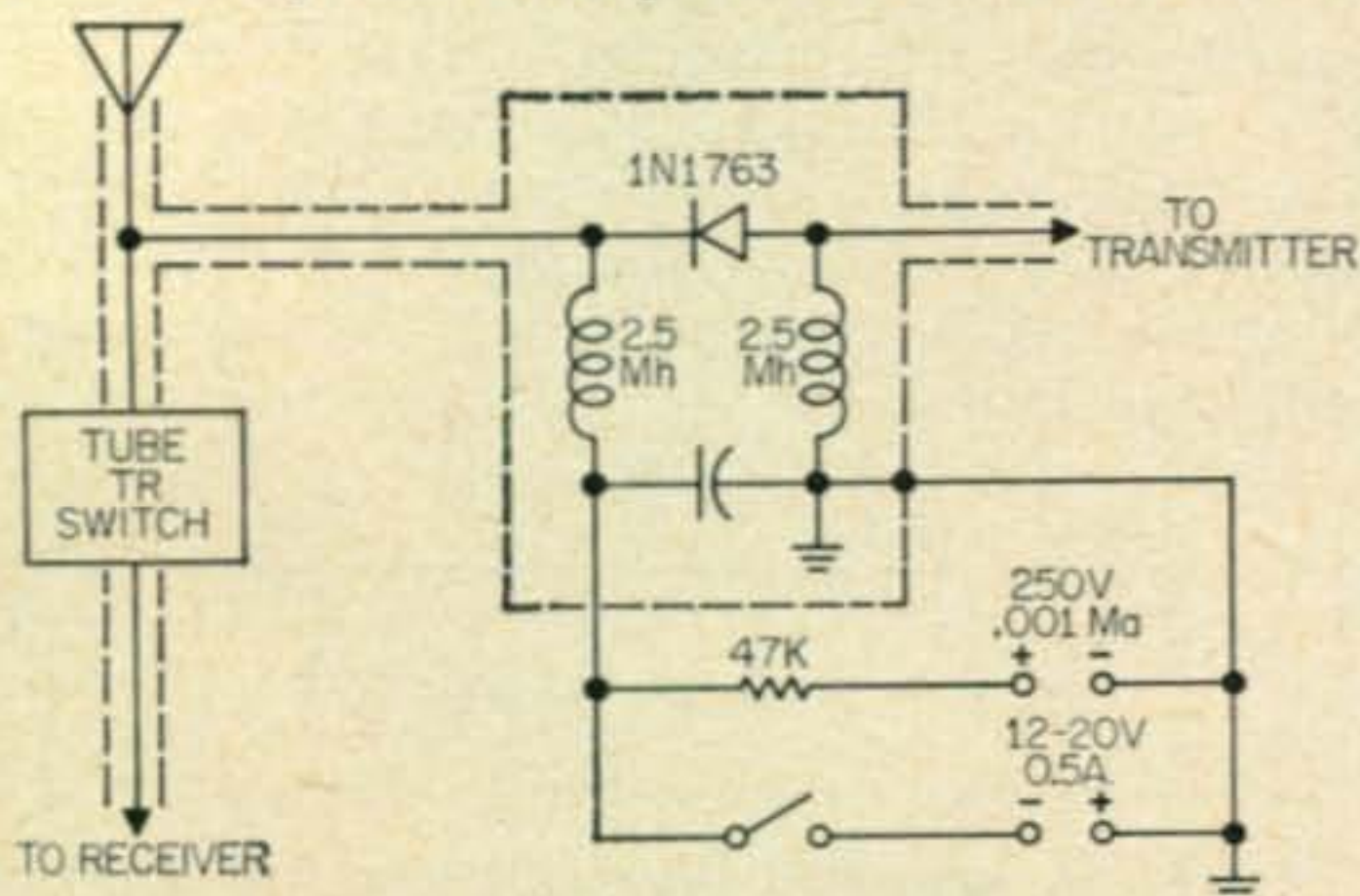
Fig. 5—A power diode may be used to make or break the connection from the antenna to the transmitter to prevent "suck-out."
