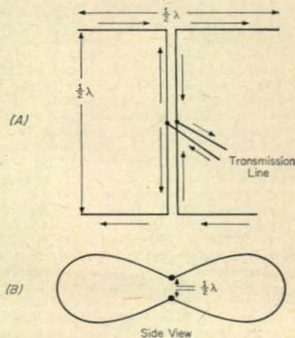
Fig. 6—Two element broadside array and its resultant vertical radiation pattern.
