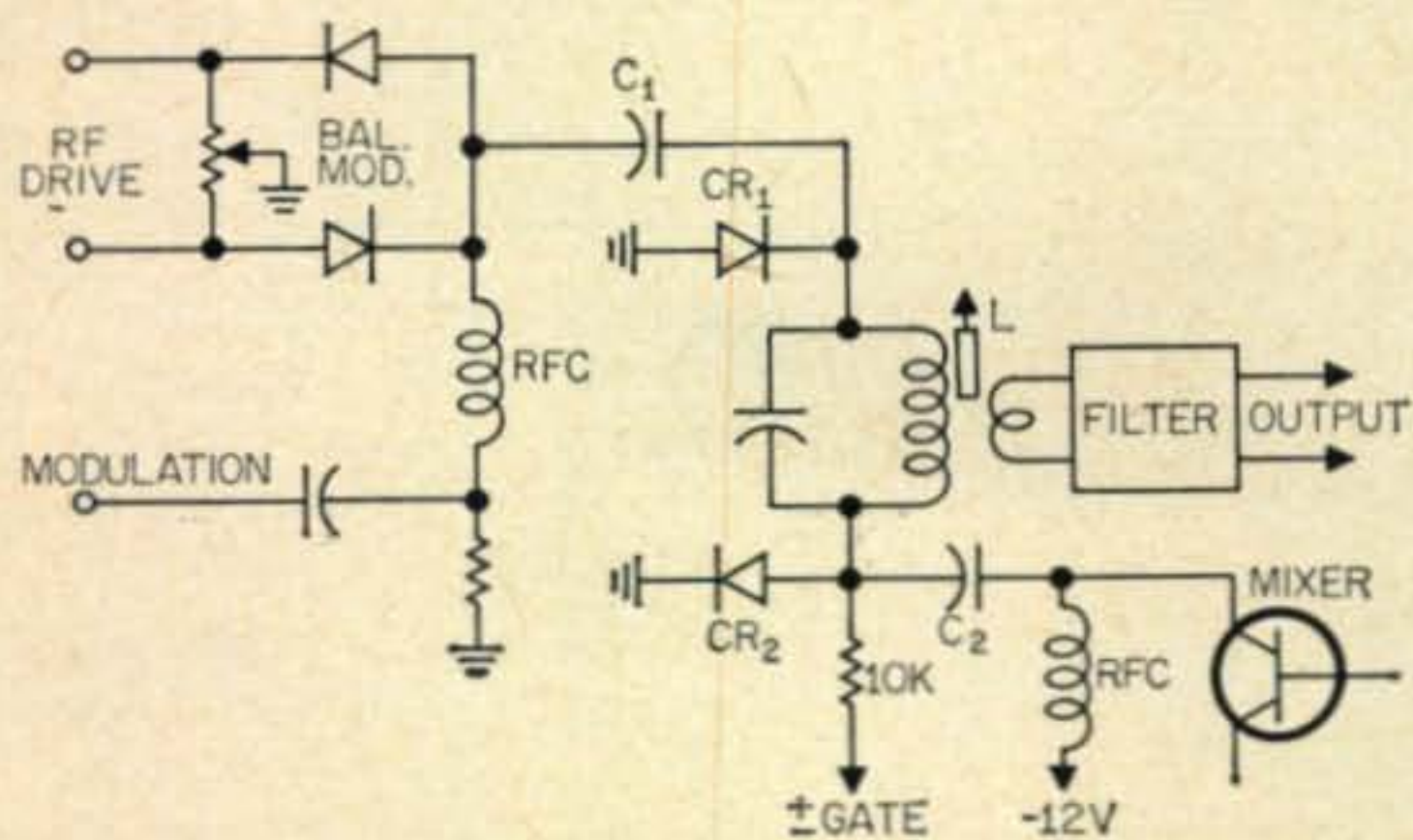
Fig. 6—A diode signal switcher for transistor circuits. Two diodes allow an ssb filter to be duplexed on receive and transmit. A similar system would be used at the output of the i.f. strip.
