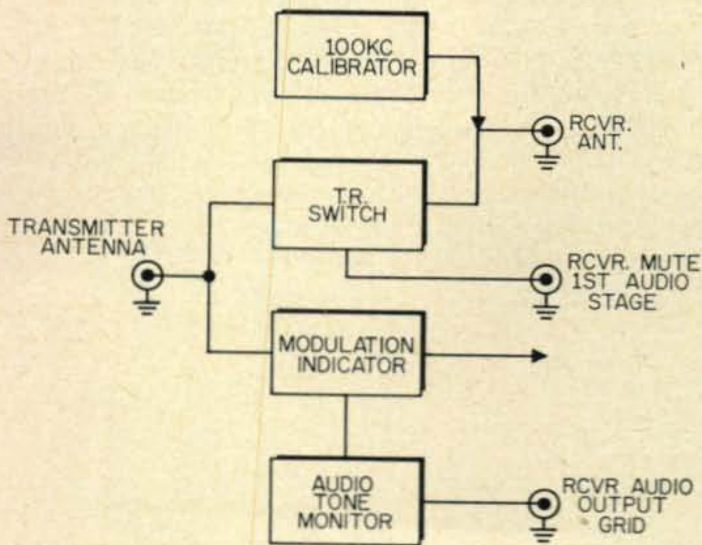
Fig. 3—Block diagram of the "Electronic Control" unit.
