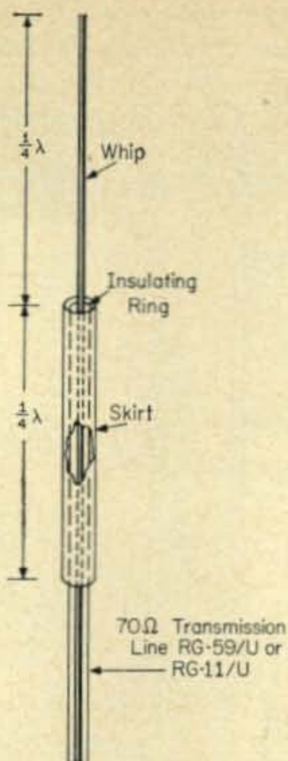
Fig. 1—Coaxial or sleeve antenna. The inner conductor of the transmission line is connected to the whip. The outer conductor is connected to the skirt. The whip and skirt are separated by an insulating ring.
