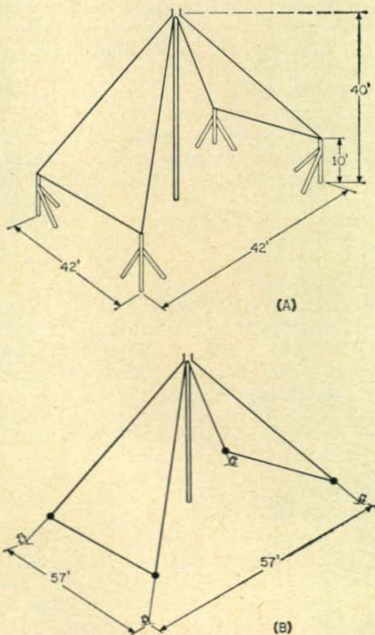
Fig. 3—Two alternate methods of anchoring the corners of the Pyramid. Method (A) would be more suitable for a small lot.
