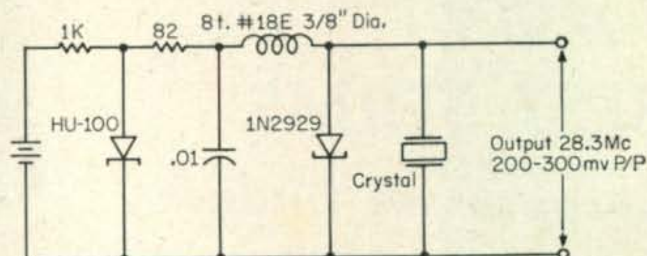
Fig. 3—Tunnel diode transmitter for 10 meters.
