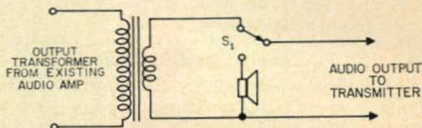
Fig. 2—Method of obtaining audio output without disturbing audio amplifier. S 1 is a single pole double throw switch which allows the audio to be switched from the existing speaker to the transmitter.
