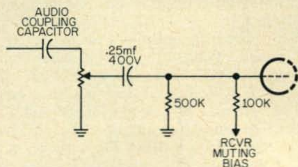
Fig. 2—Muting bias voltage divider in receiver. This also provides isolation for hum as described in the text.
