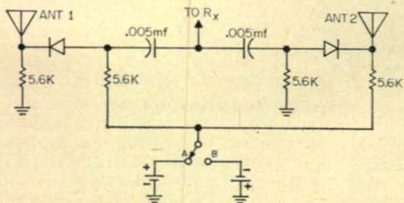
Fig. 3—A SPDT diode switch. Diode sections may be ganged together giving any desired combination of switching.
