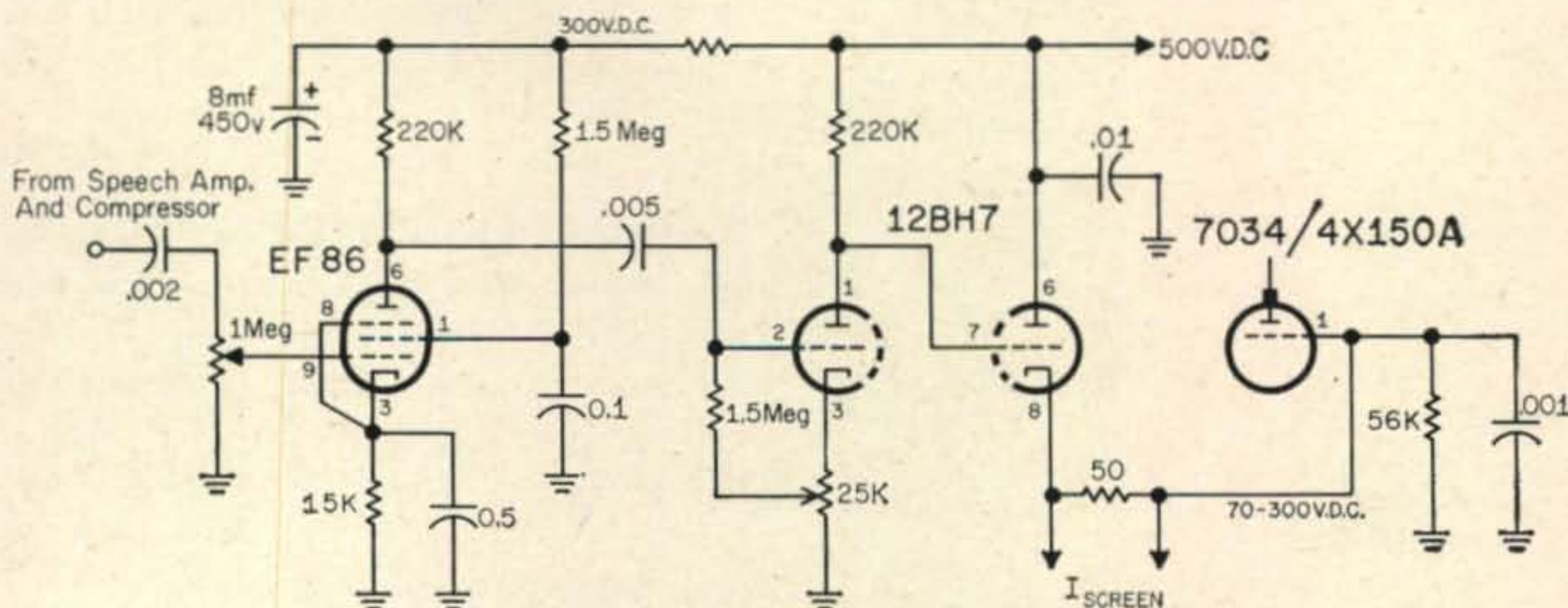
Fig. 2—Schematic of the gated screen controlled carrier modulator used in the T-400 transmitter.
