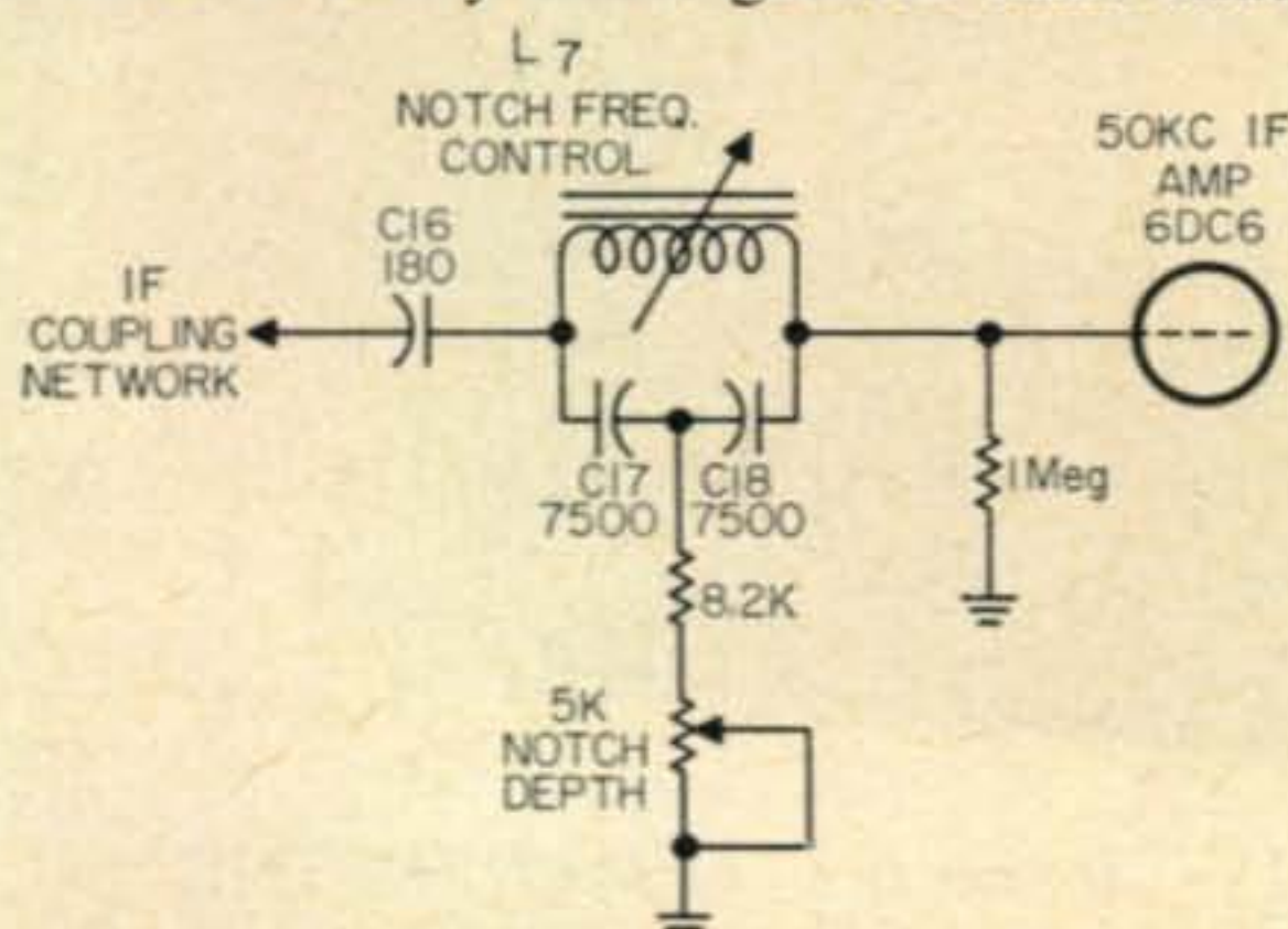
Fig. 4—Diagram of the notch-filter in the SX-111. The notch frequency is controlled by inductor L 7 , while the notch depth is controlled by the 5K potentiometer.
