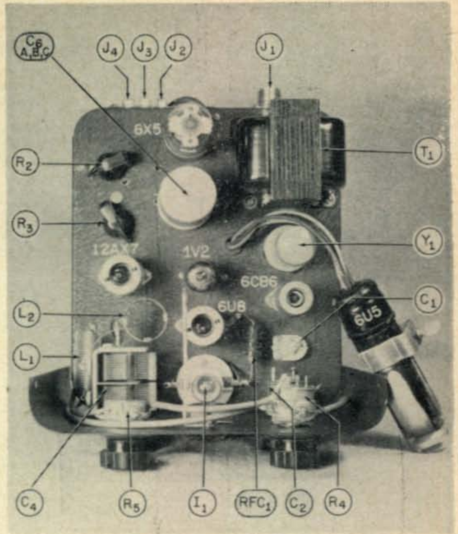
Top view showing component layout and identification.
