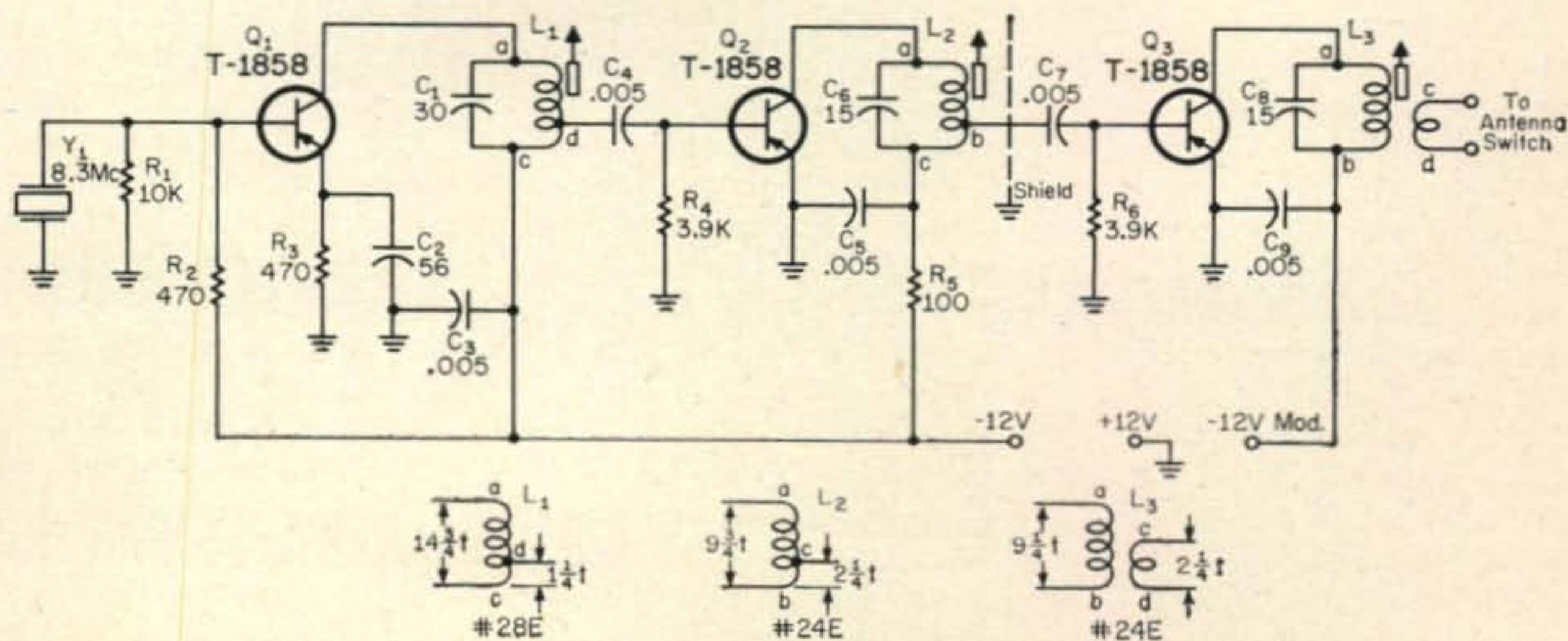
Fig. 2—Six meter transmitter circuit. Coils L_1 , L_2 and L_3 are wound on \frac{1}{4} " slug tuned forms.
