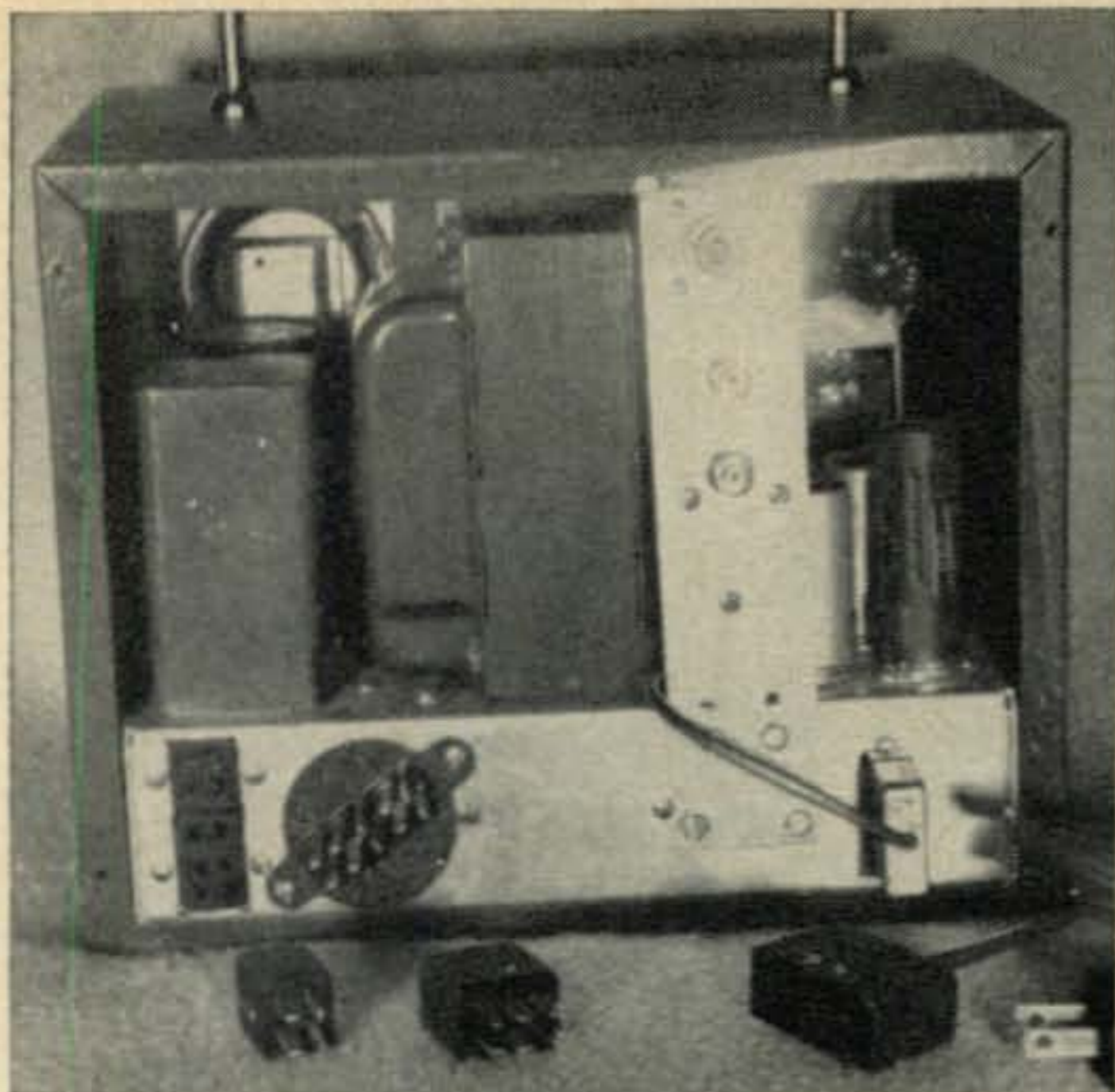
Rear view shows the "programming" plug arrangement on the left. On the right of the chassis is the v.f.o. plug made from an old surplus crystal holder. The vertical bracket contains the three antenna connectors.
