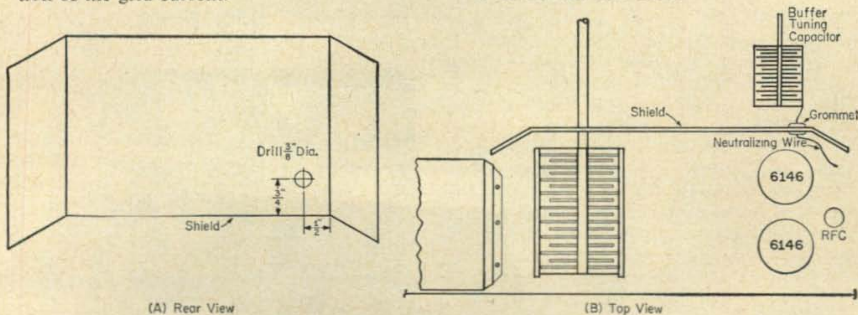
Fig. 4-A: Location of the hole in the interstage shield which permits the neutralizing lead to perform its function. Insert a rubber grommet in the \frac{3}{8} " hole. B: Solder neutralizing wire to the stator of the buffer tuning capacitor. See text for adjustment.
