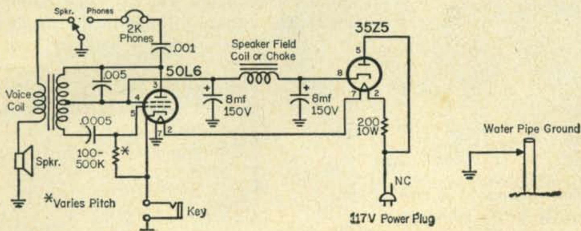
Fig. 4 — A two tube code practice oscillator designed by John Creamer, KNØBVR. If the tubes do not light, simply reverse the plug in the wall.
