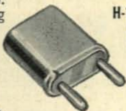
H-17TL (HC-13/U). Pin Dia. .090". Pin Spacing .468"
