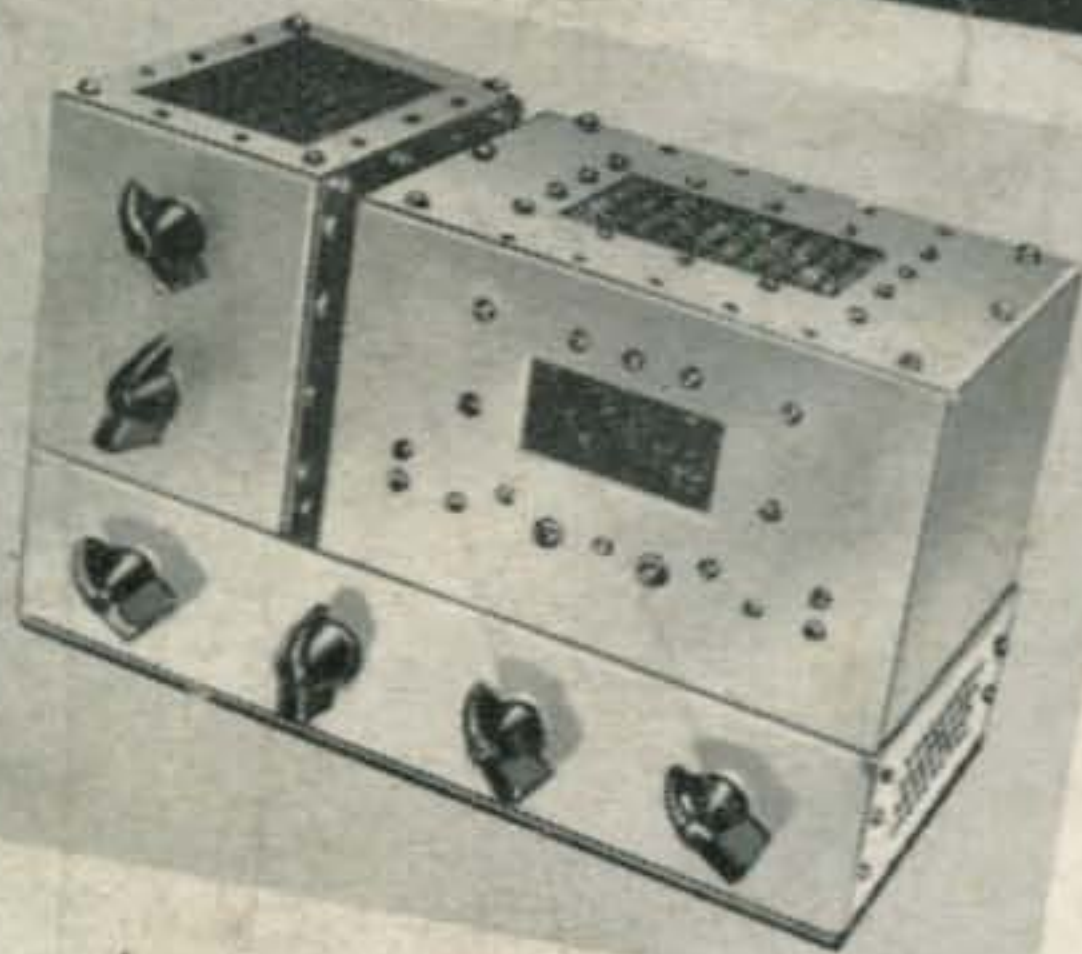
Front view of the 50 mc exciter showing arrangement of tuning controls and three major elements of the unit. Controls, from upper left to lower right are: 6146 plate tuning, antenna loading, meter switch, 5763 plate tuning, 6AG7 plate tuning and crystal f.o. switch. The 4 x 3 x 6" utility cabinet on the right houses the crystals, low level preamp, meter and clamp tube. The left hand utility cabinet 3 x 4 x 5" houses the 6146 r.f. amplifier circuit components. The basic chassis is only 5 x 9 1/2 x 2".
