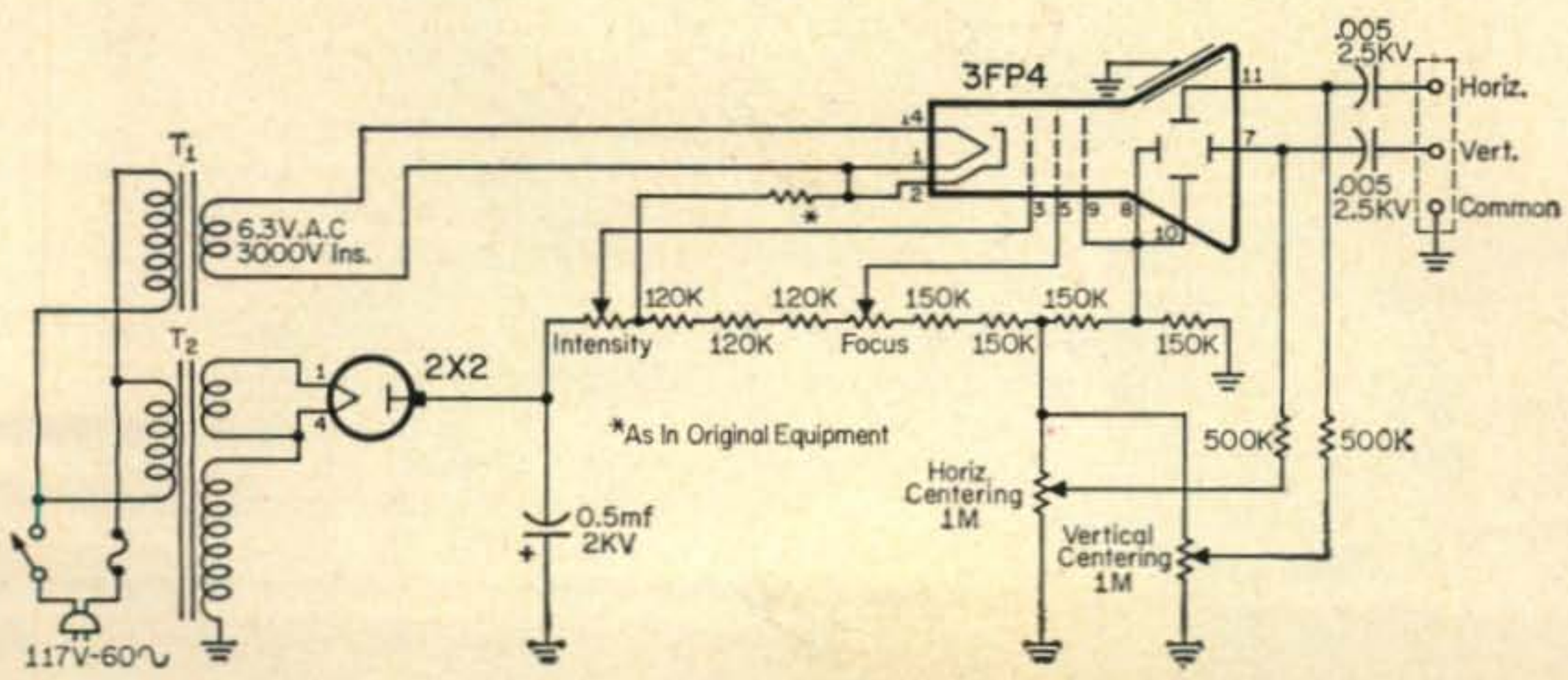
Fig. 1—Power supply and modified bleeder circuit used with APS-4. The amplifiers (horizontal and vertical) remain unused.
