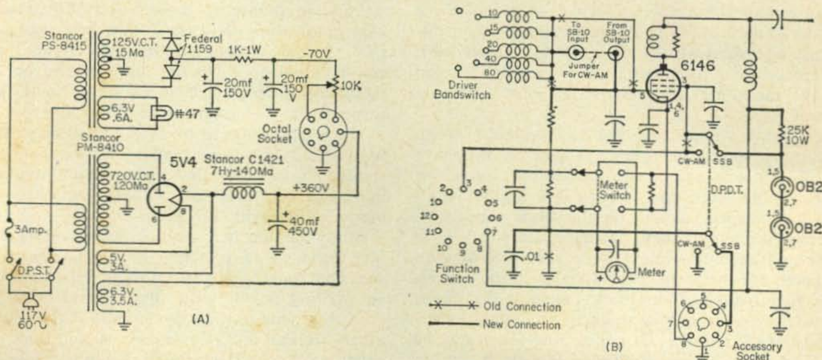
Fig. 1—(A) Power supply suitable for use with the Heath SB-10 and DX-40. (B) Diagram illustrating changes necessary in the Heath DX-40 for use with the SB-10.
