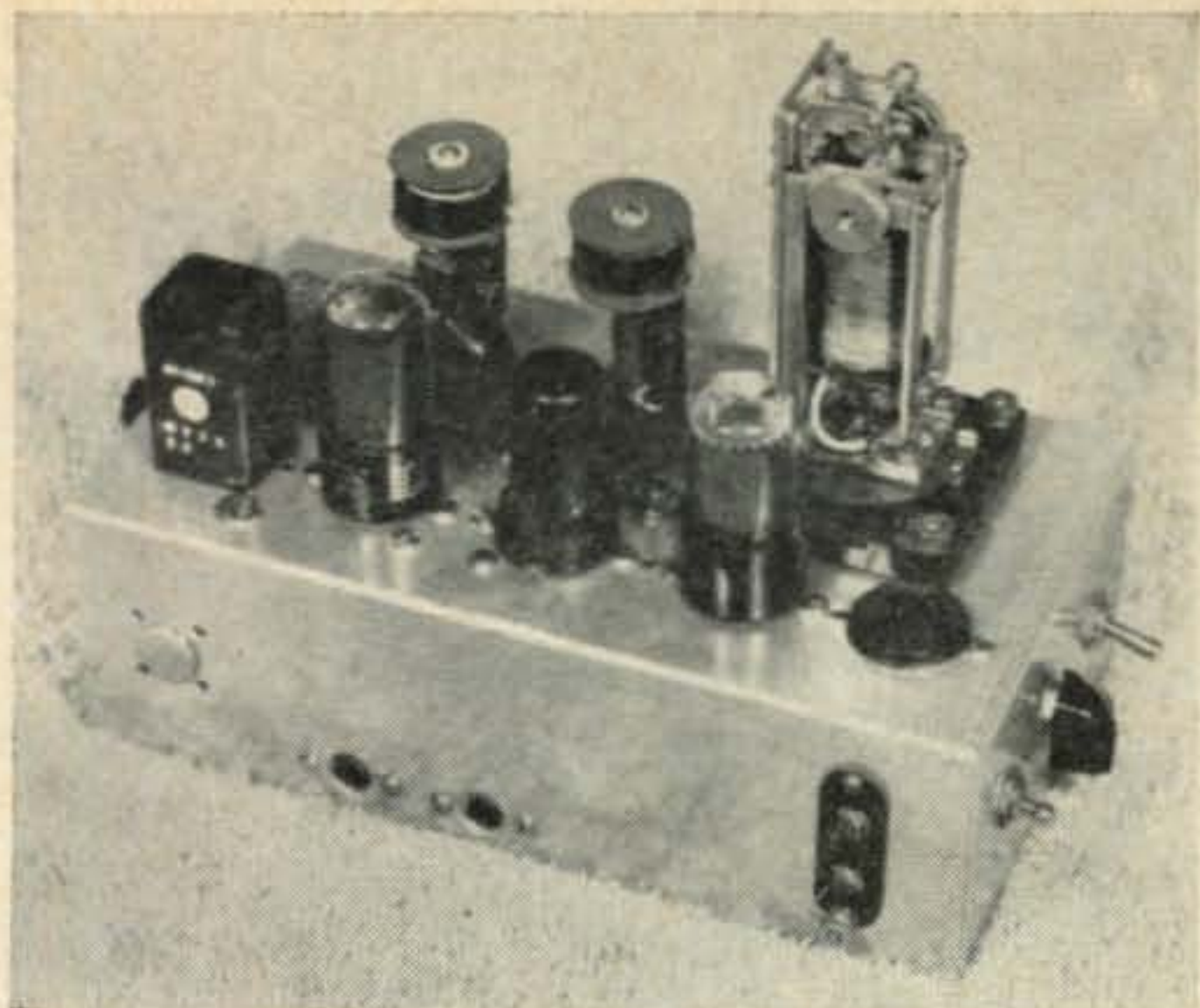
The Twin City TU, a simple RTTY converter.
