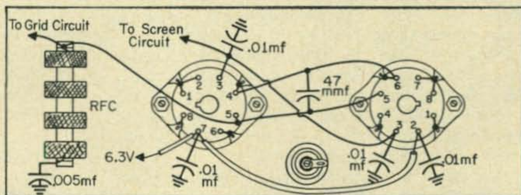
Fig. 2—Pictorial representation of the sub-chassis wiring at the 6146 sockets.
