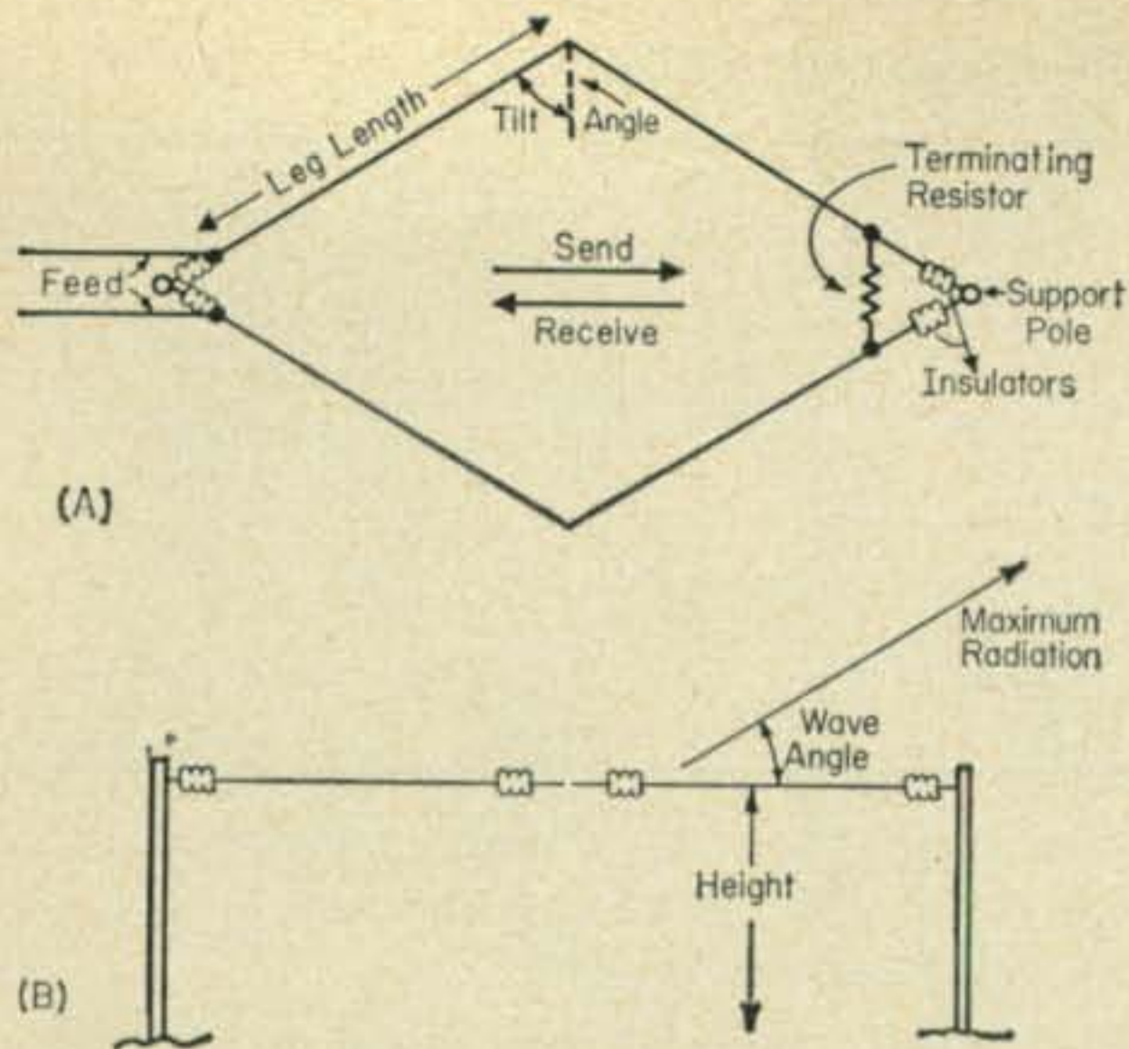
Fig. 6—The ultimate in long wire antennas, the terminated rhombic, showing wave and tilt angles in side and top views.
