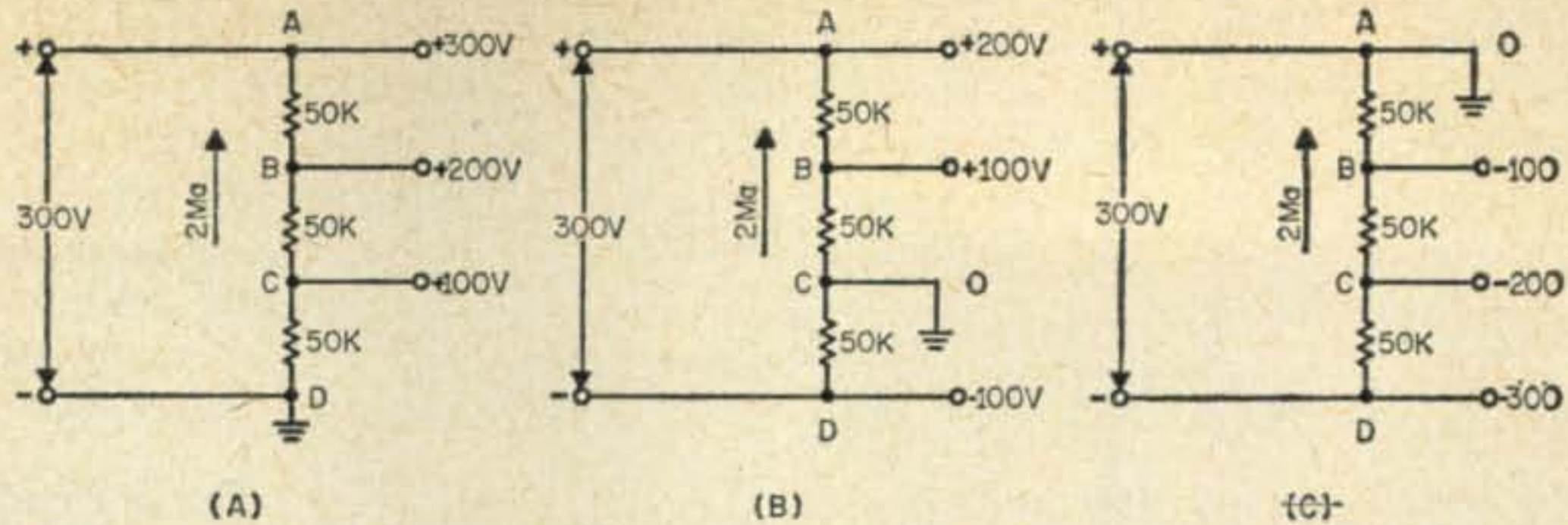
Fig. 2 — Ground or common is an arbitrary word. It can be placed anywhere in a voltage divider circuit to supply a variety of output voltages and polarities.
