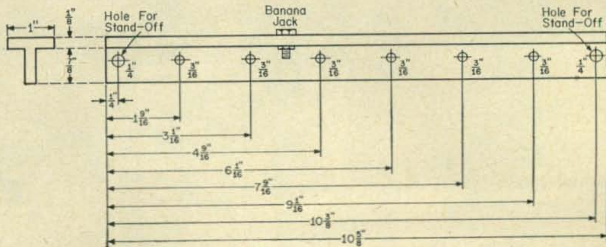
Fig. 2—Layout of holes for mounting the resistors on the 1/4" thick "T" angle. Two such pieces are required.
