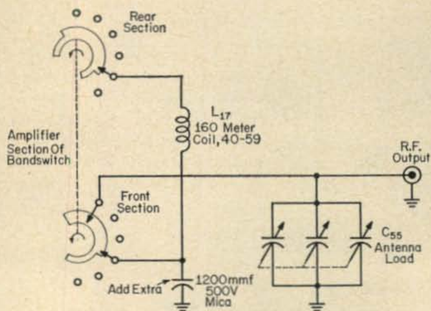
Fig. 1—A one-sixty loading capacitor may be mounted between the "cold" terminal of the 160 meter coil (terminal nearest 6146 sockets) and the ground bus of the variable loading capacitor. Refer to page 2 of the DX-100 manual for the complete schematic.
