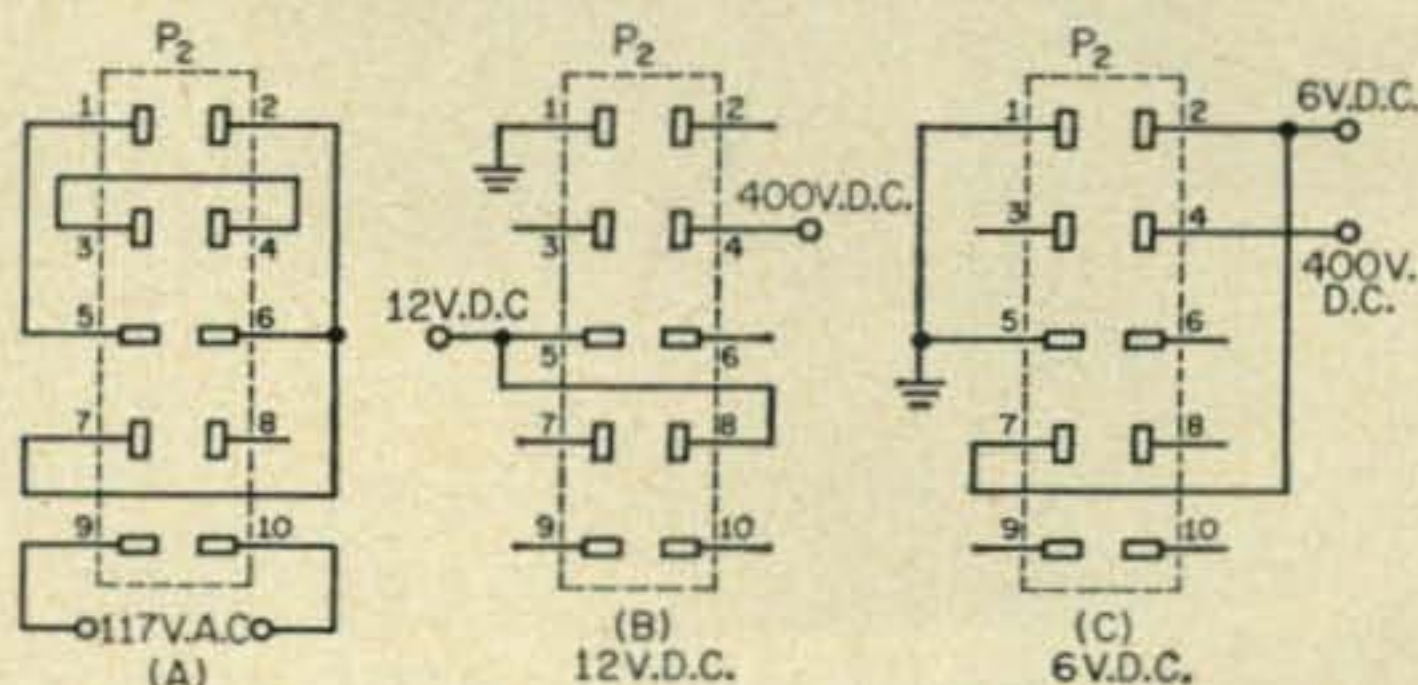
Fig. 3—Jumper plug P_2 connections for various methods of operation. (A)—Plug for the use of self contained a.c. power supply. (B)—Plug for 12 volt external filament supply and separate high voltage source and (C)—Plug for 6 volt filament supply with external high voltage supply.
