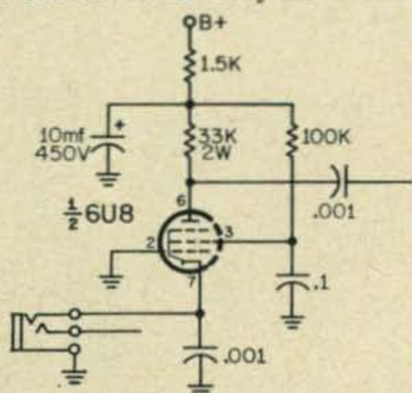
Fig. 2—Schematic illustrating the changes necessary in the speech amplifier circuit of the "All Around" for use with carbon microphones. The original 6AN8 is replaced with a 6U8 with appropriate changes in pin connections in both sections.
