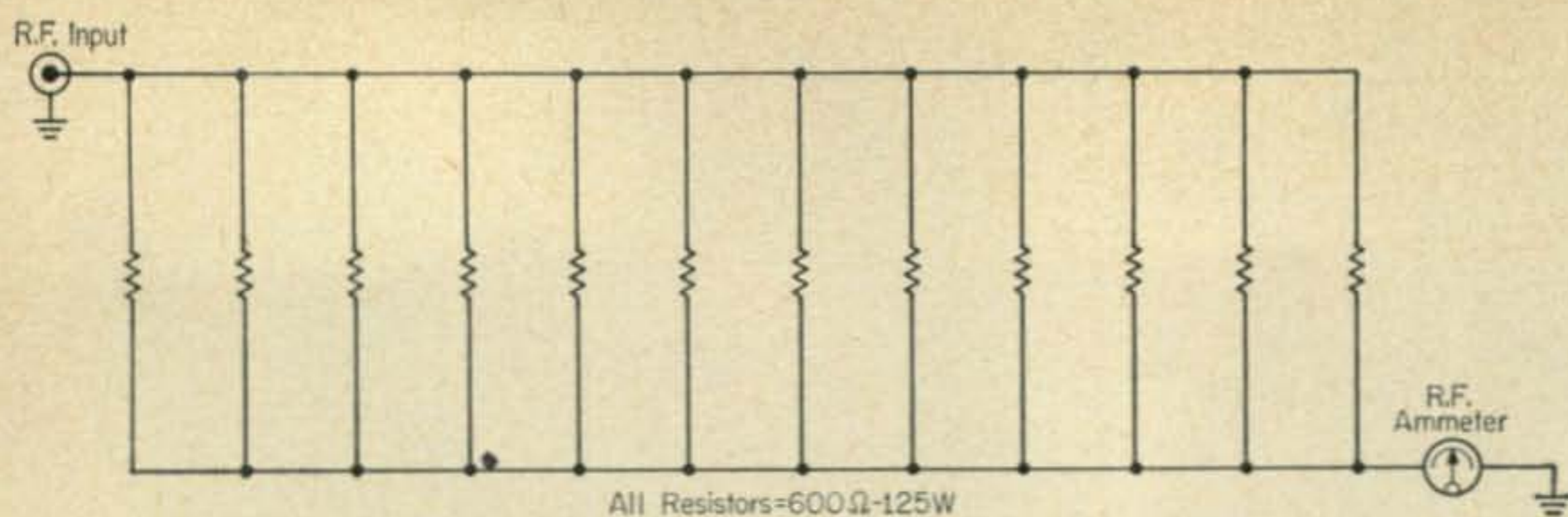
Fig. 4—Simple circuit of the 1500 watt dummy load using inexpensive high power, non-inductive resistors, available surplus.
