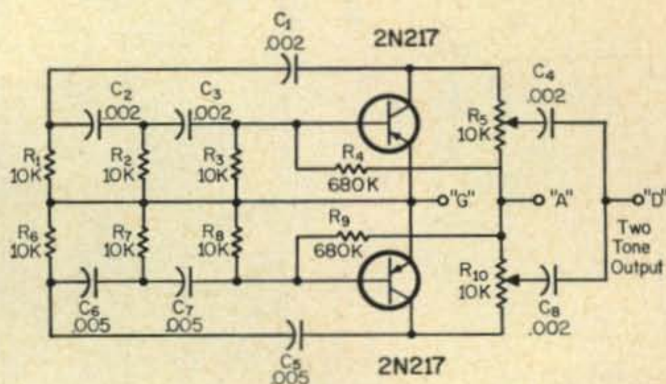
Fig. 2—A two-tone audio oscillator for s.s.b. exciter alignment. For best results, a 22.5 volt battery should be connected between "G" (positive) and "A" (negative). Output is taken between "G" and "D".
