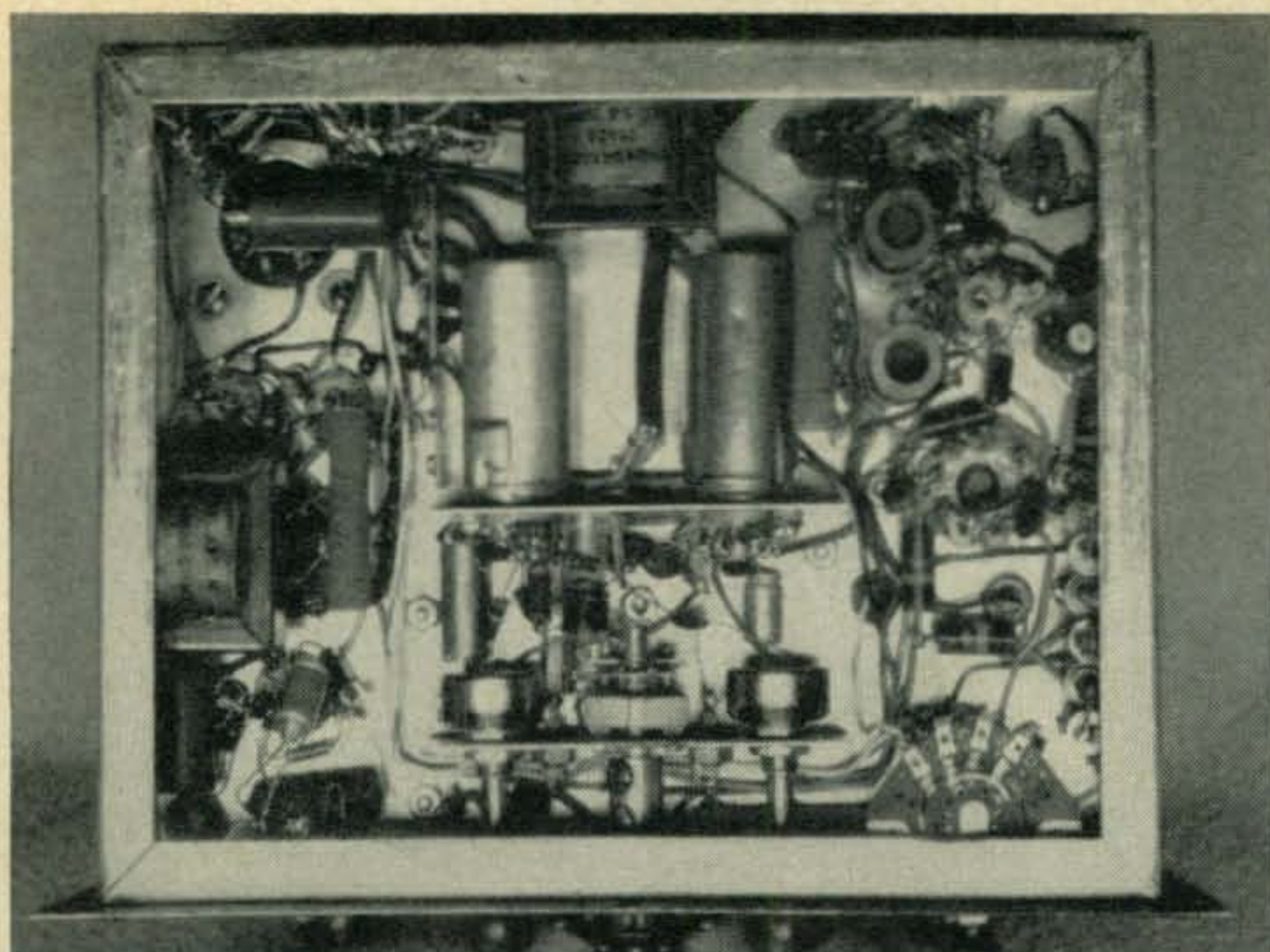
Under-chassis view of the ten meter transmitter-receiver. The receiver components are mounted on two angle brackets. The tubes and tuning controls are so arranged that the shortest possible leads are obtained.
