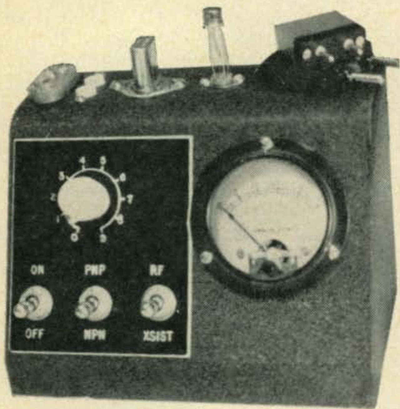
Front view of Stuart C. Rockafellow's transistor and crystal tester.
