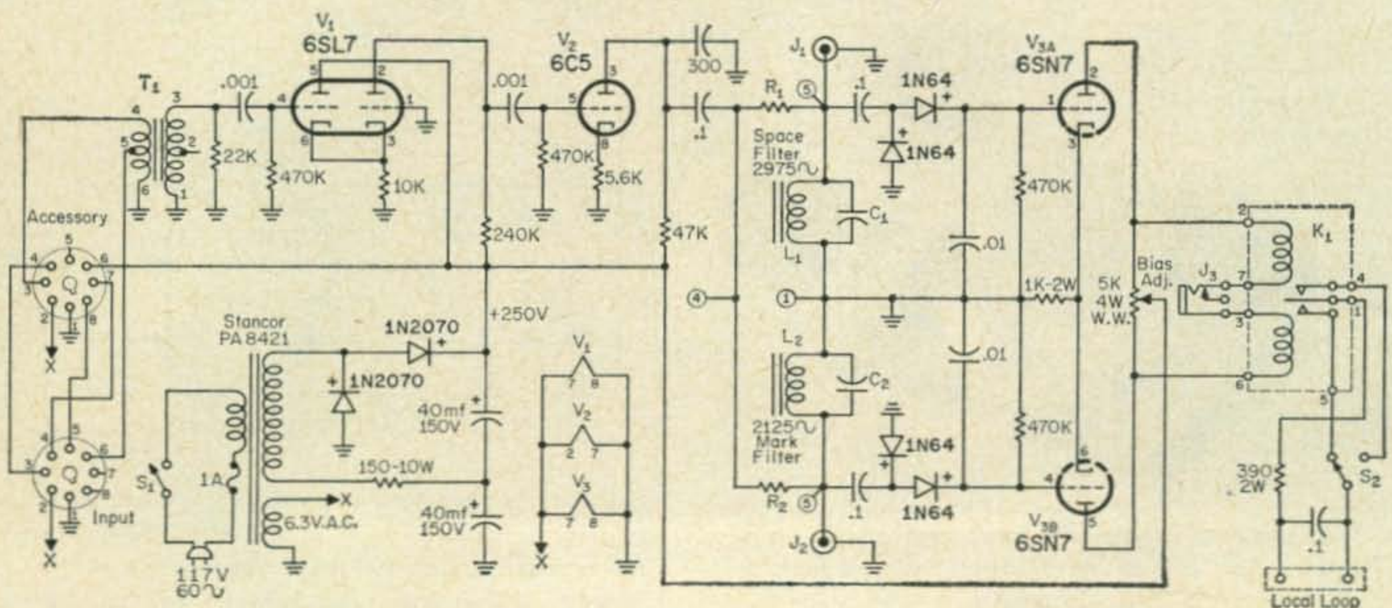
Fig. 1—Schematic diagram of the Twin City TU.
