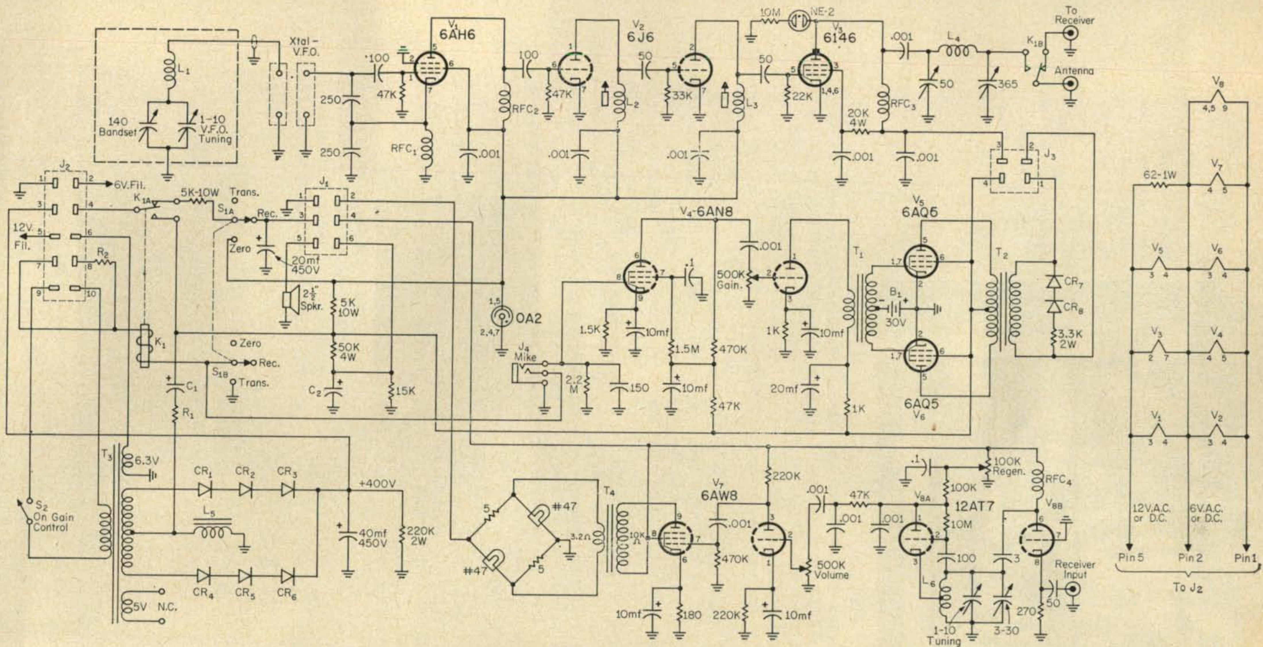
Fig. 1—Complete schematic of the "All Around" portable 10 meter station.
