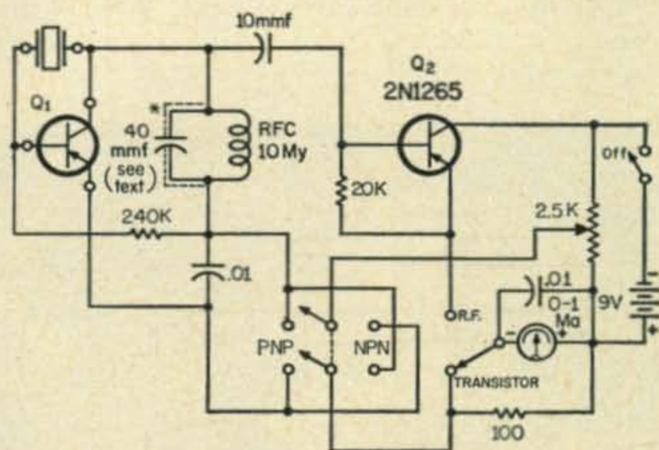
Fig. 1—Schematic diagram for the crystal and transistor tester by W8NJH. The PNP-NPN switch is a double-throw, while the switch used to connect the meter for r.f. or current measurement is a single-pole, double throw type.
