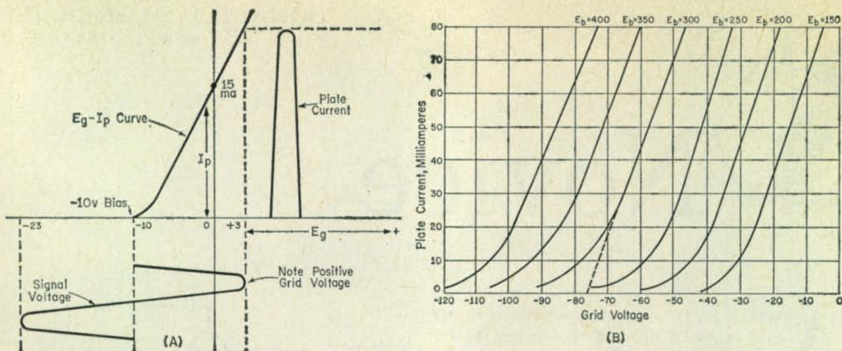
Fig. 2 — A Class B amplifier operates over only one half of the applied cycle. The E_g-I_p curve can be used to determine the proper operating point for the Class B stage as explained in the text.
