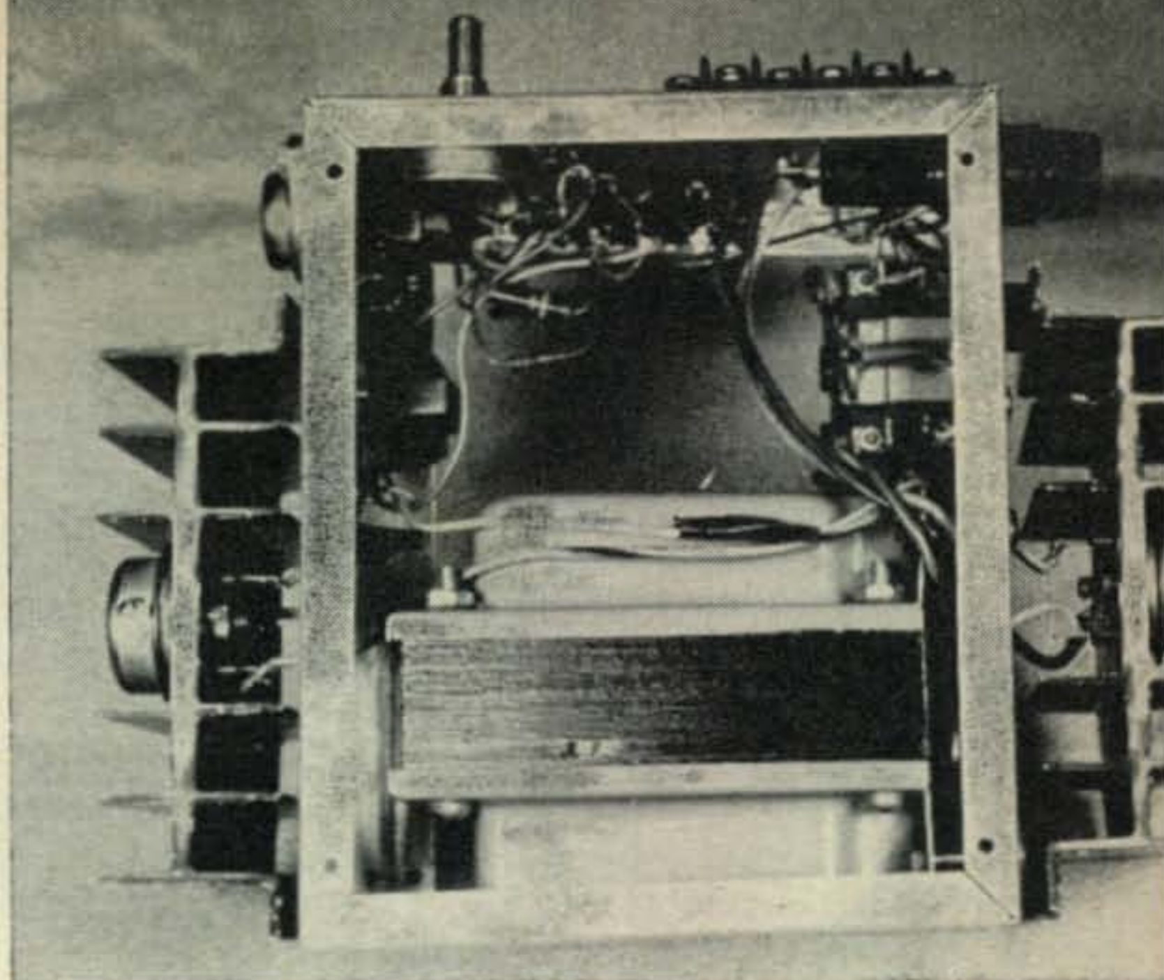
Bottom view of the transistorized modulator shows T_3 occupying the bulk of the internal space. Relay K_1 is on the right front chassis flange and transformers T_1 and T_2 are in the front left section of the chassis.
