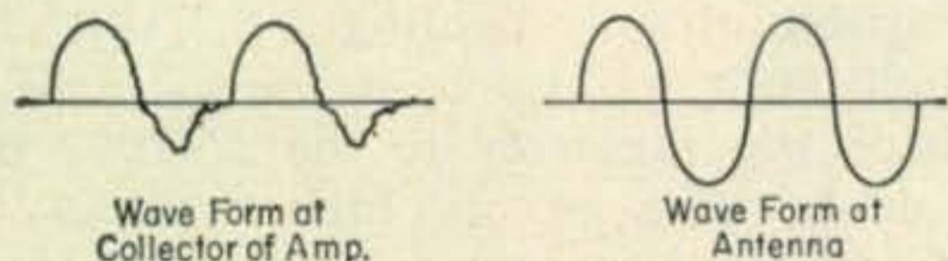
Fig. 3. The two tuned circuits are necessary at the output to put back the missing half cycle.
