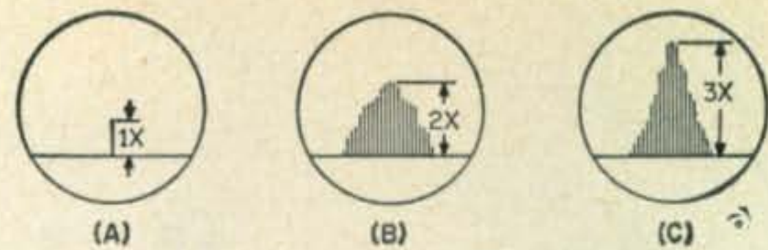
Fig. 3—Panoramic adaptor displays comparing the output of standard a.m. to Taylor Modulation. A—Unmodulated carrier. B—100% amplitude modulation. C—100% Taylor Modulation.
