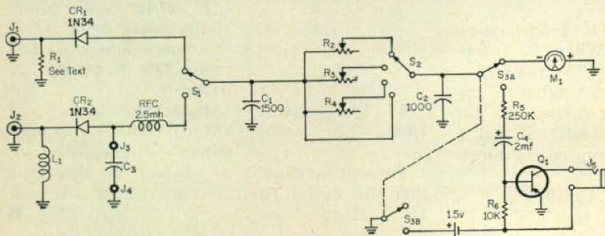
Fig. 1—Circuit of the Handy Dandy transmitter checker. Inductor L_1 is on r.f.c. and a tank circuit may be used if a specific frequency is desired.
