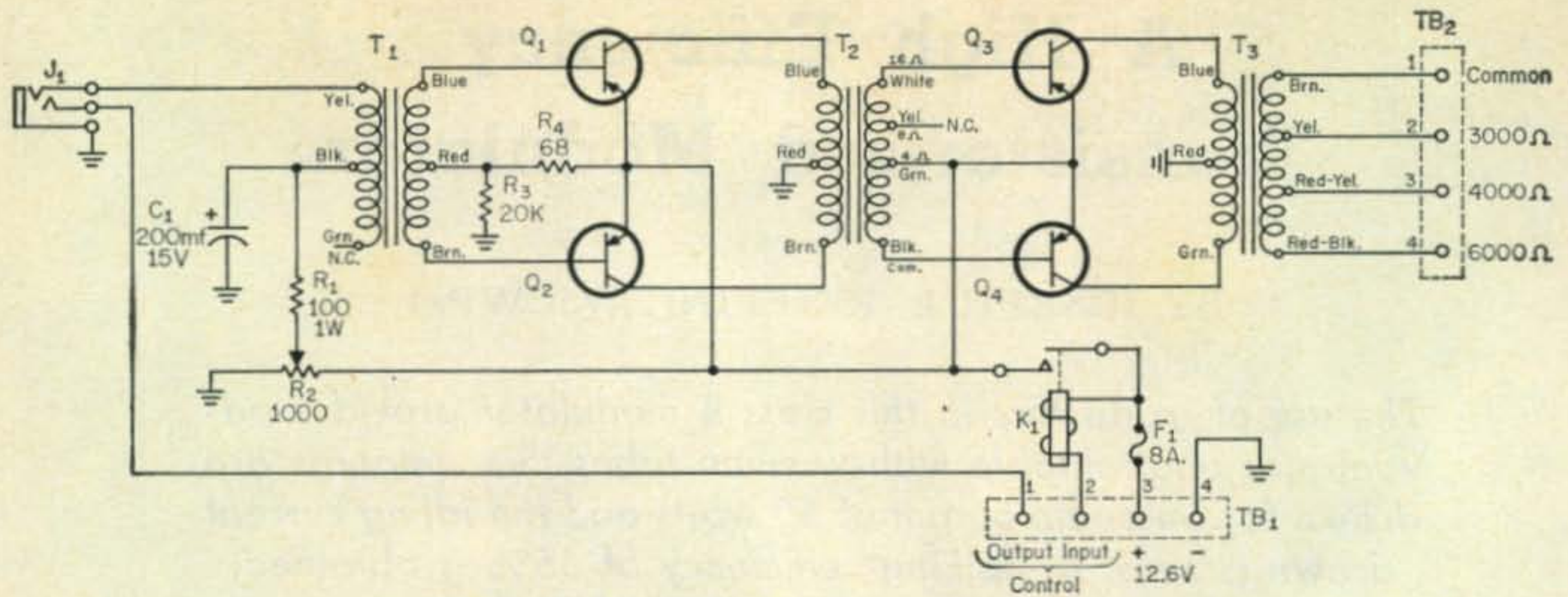
Fig. 1—Circuit of the high efficiency transistorized modulator.
