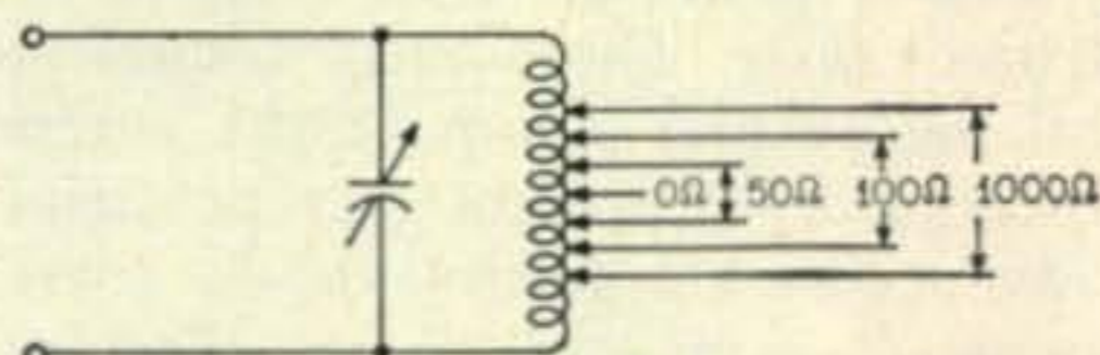
Fig. 3—Illustration of the relative impedance tap positions on a coil. The lowest practical value, without a vernier coil, is about 50 ohms.
