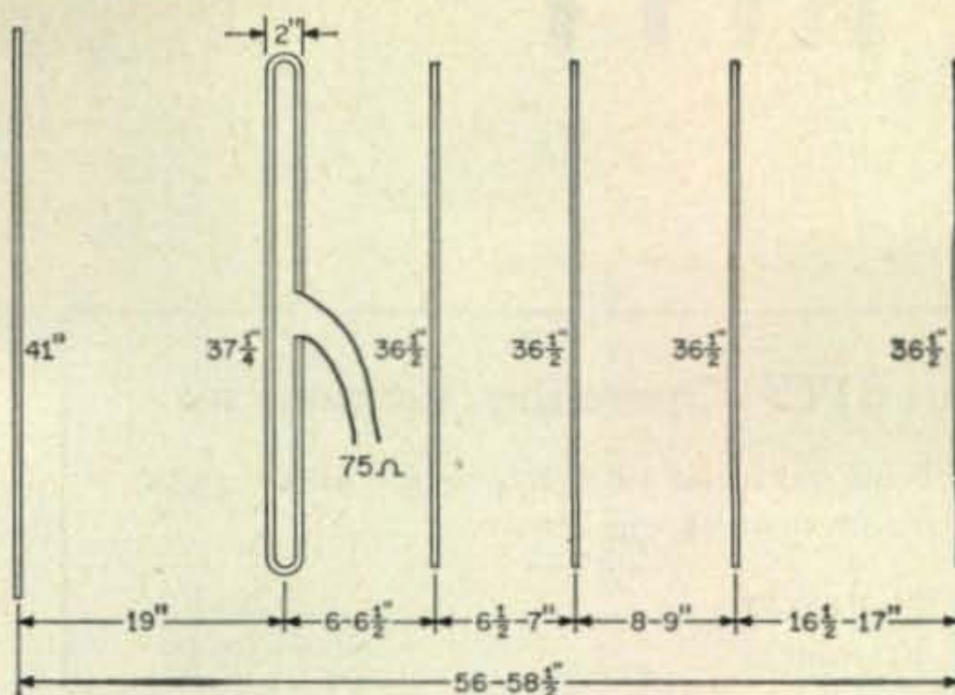
Fig. 2—G2DHU's 6 element 2 meter beam constructed of 1/4" aluminum rods. Element spacings are not critical and may vary between the limits shown.
