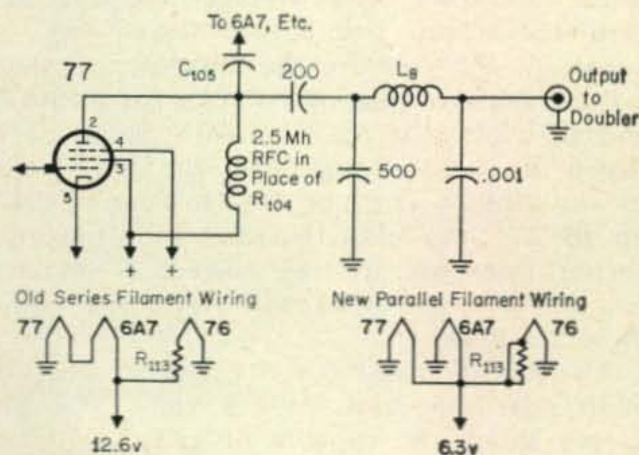
Fig. 8—Modifications made in the filament and output circuit of the LM so that it may be used as a v.f.o. This does not preclude its use as a frequency meter also. Inductance L_8 is 22 turns of #22E, 1" diameter, 1" long.
