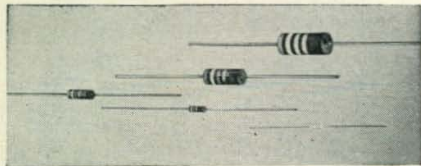
Typical molded composition resistors manufactured by Ohmite. The resistors are rated at 1/10, 1/4, 1/2, 1 and 2 watts. (Photograph courtesy of the Ohmite Manufacturing Co.).
