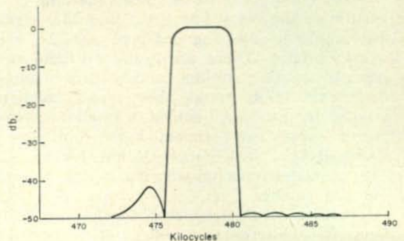
Fig. 10—Response curve of the 480 kc i.f. when properly adjusted.
