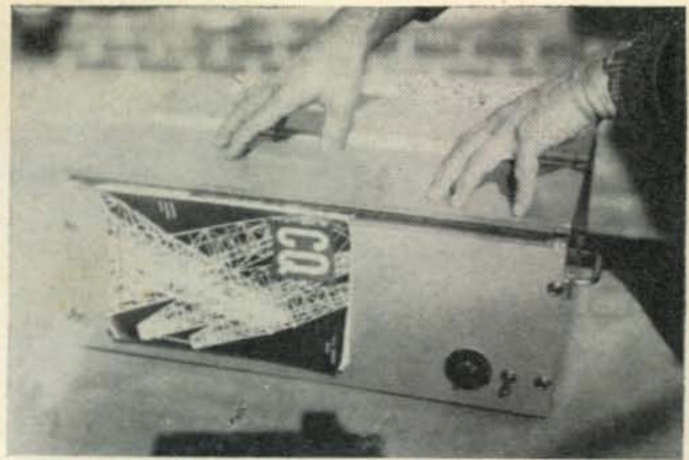
Front view of the light box. The cover is split and fastened with a piano hinge to facilitate duplicating smaller size copy.
