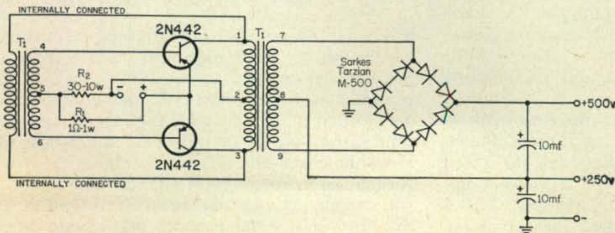
Fig. 5—Circuit for a transistorized d.c. to d.c. converter as suggested by the Microtran Co. Transformer T_1 is the Microtran M8035.
