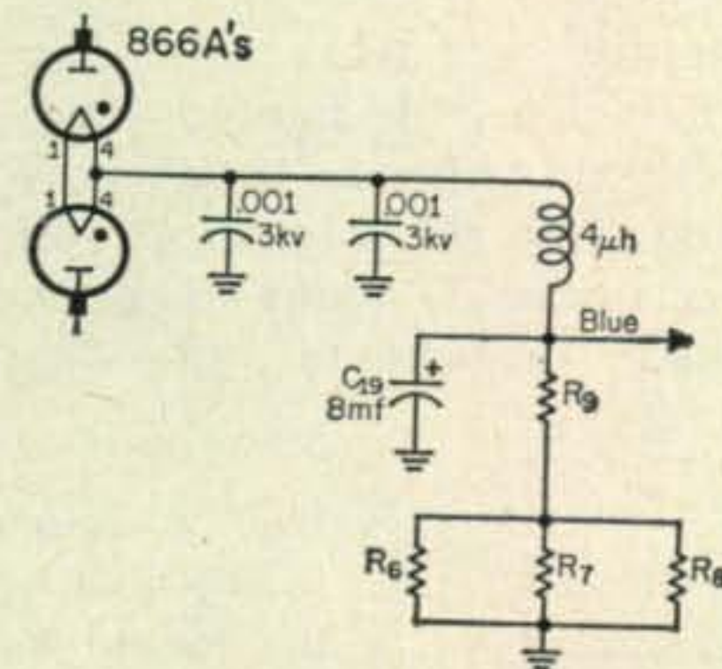
Fig. 4—Circuit for the suppression of mercury vapor rectifier hash in the Heath Warrior amplifier. The 866A filaments should be wired as shown and high voltage taken from pins 4.
