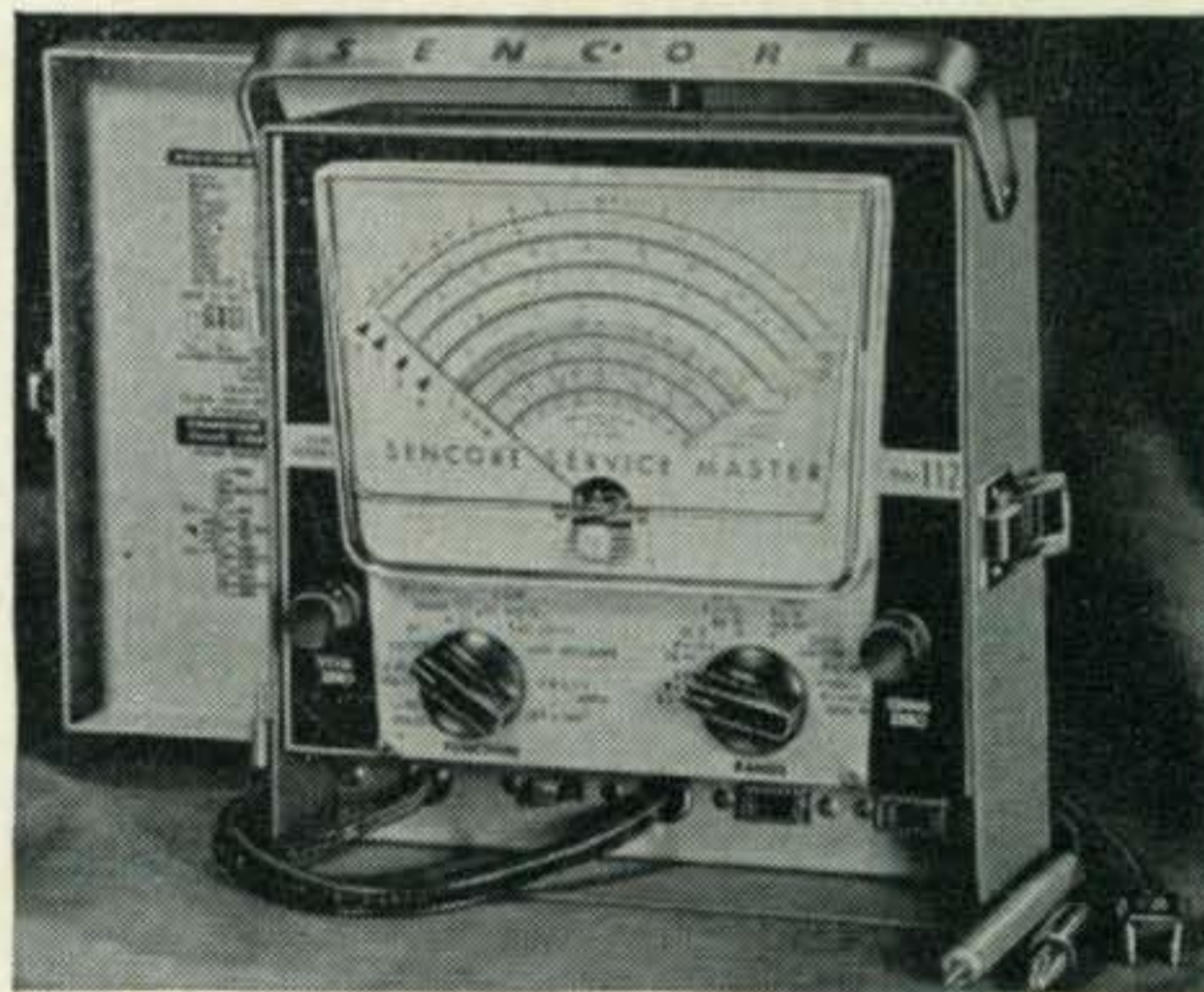
Sencore combination VOM-VTVM.
