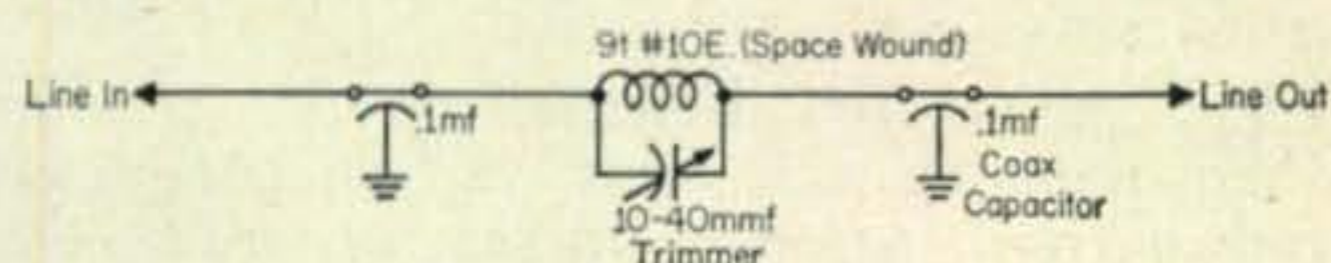
Fig. 8—Parallel resonant trap for eliminating rotator noise radiation on 10 meters. Other similar units may be necessary for 20 and 15 meters.
