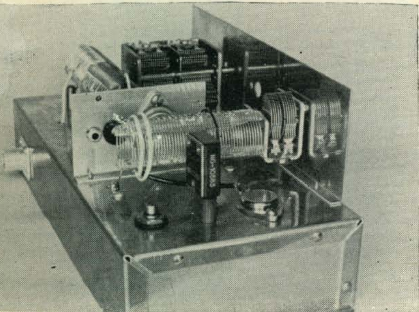
The PADT50 is shown mounted to the right of the crystal. The transistor is insulated from the chassis with a mica washer. The 2N1907 can be seen behind the oscillator coil in the foreground.
