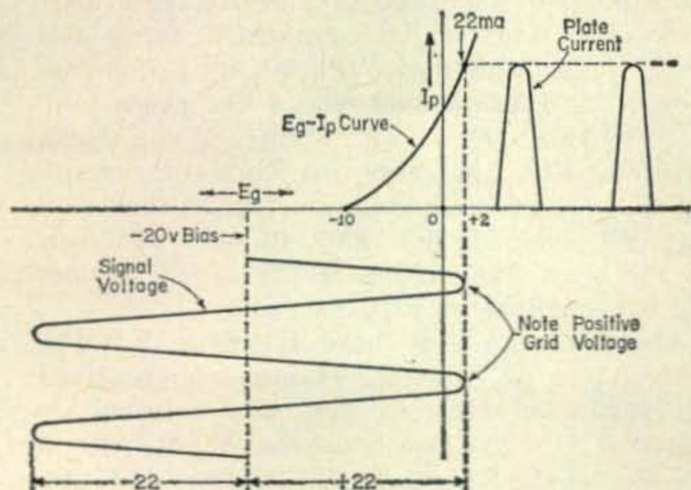
Fig. 5 — In Class C, the grid is biased beyond cut-off and the tips of the r.f. positive half cycles kick the tube into conduction.
