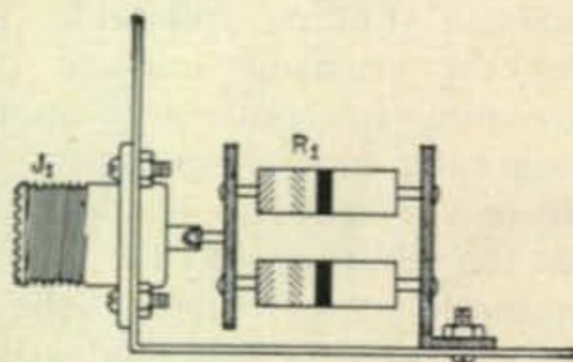
Fig. 2—Details of the dummy load construction.
