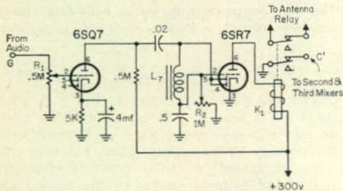
Fig. 9—Circuit of the vox stages. The audio signal, applied to G, is obtained from point C in fig. 2. Controls R_1 and R_2 adjust operating threshold and hold time.
