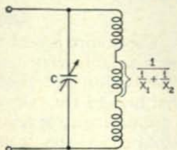
Fig. 2—The parallel circuit, X_1 and X_2 , results in a reduced overall inductance that can be compensated for by C.
