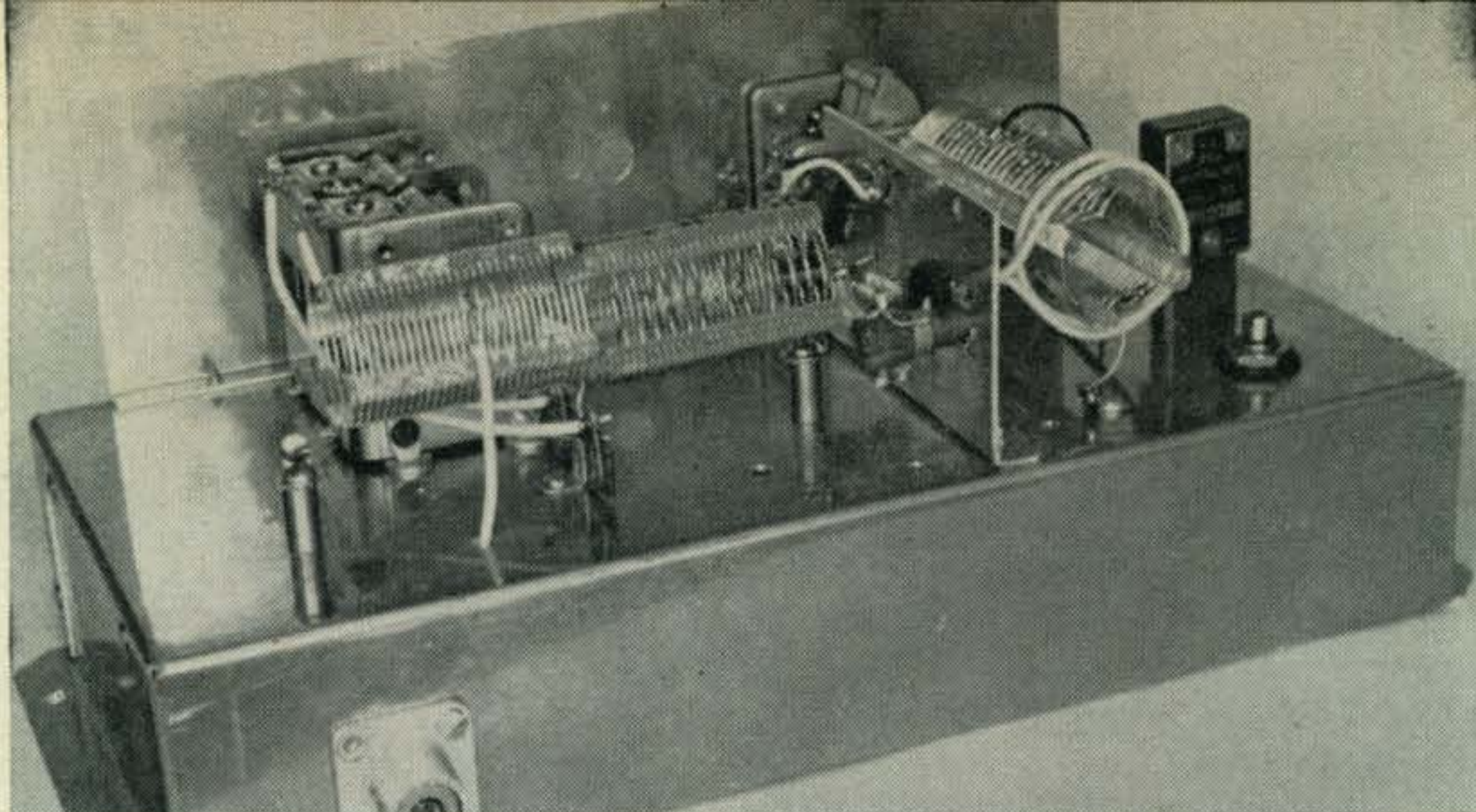
Rear view of the r.f. amplifier showing bandpass coupler coils and the neutralizing coil L_n . No transistor sockets were used in this rig. Wires are soldered directly on to the pin. Note the wire from the collector of the 2N1907 to the tap on coil L_2 .
