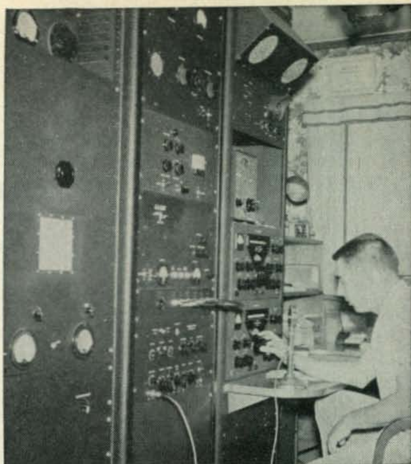
Operating position at K6QXY. Looks like he's tuning up at WMGM. Most impressive set-up with rack mounted kilowatt on the left.
