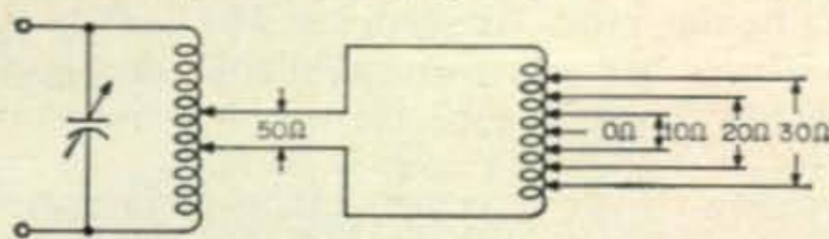
Fig. 4—Addition of a vernier coil makes possible matching impedances as low as 10 ohms.
