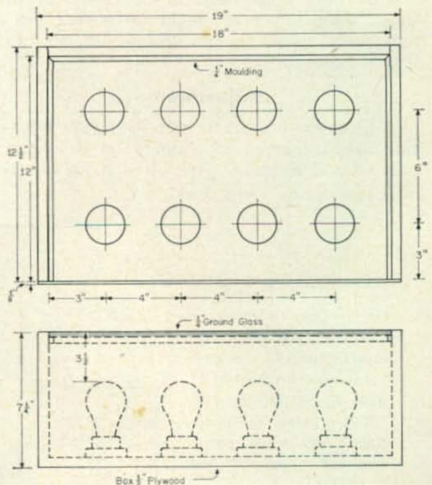
Fig. 1—Construction details for the light box. The ground glass must be 12\frac{1}{8} \times 18 \times \frac{1}{4} inches in size. The box is constructed of \frac{1}{2} " plywood and a standard relay rack panel is used for the front.
