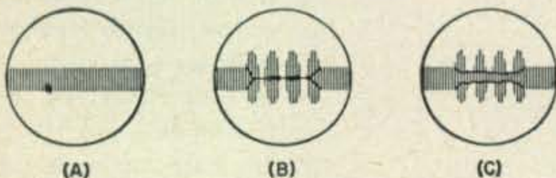
Fig. 2—Oscilloscope displays for Taylor Modulation. A—Unmodulated carrier. B—Overmodulation with some peak clipping. C—Less than 100% modulation.
