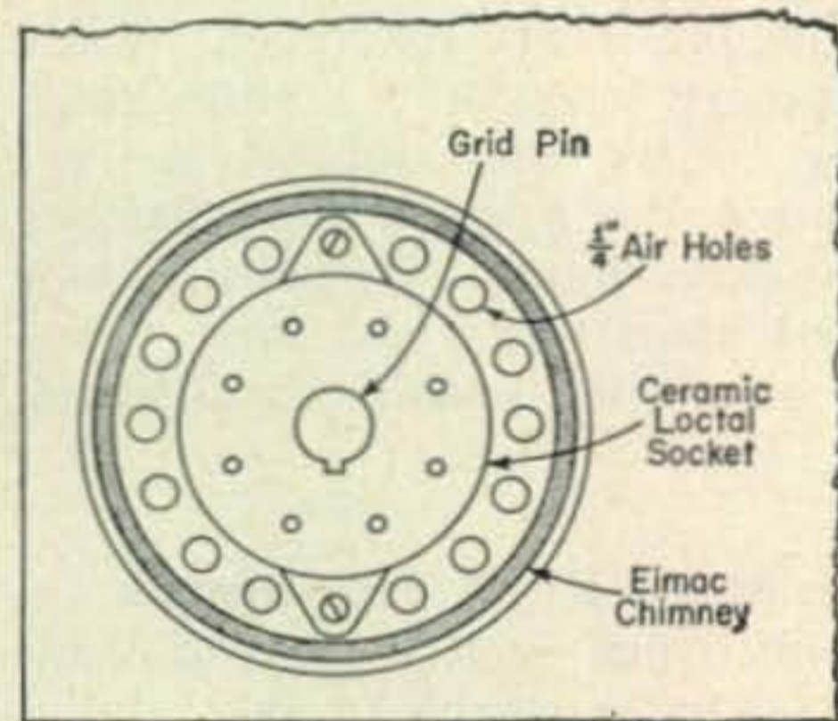
Fig. 1—Cheap and easy socket and air system for the 4X150A tubes. The ceramic loctal socket is mounted in a conventional manner on the chassis while the holes and Eimac SK-606 chimney direct air from a blower below chassis.
