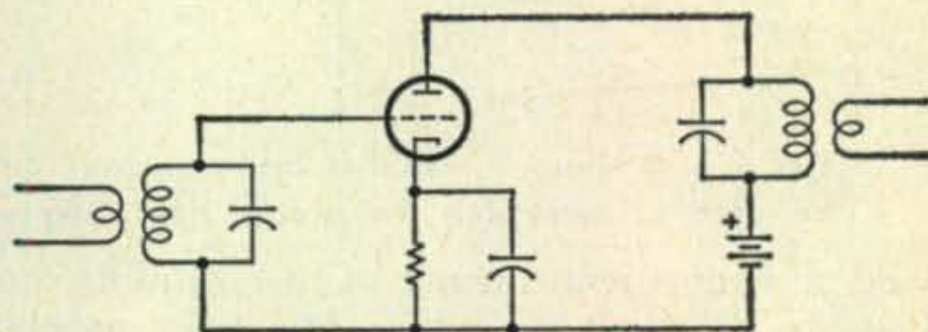
Fig. 1 — A typical Class A r.f. amplifier circuit.
