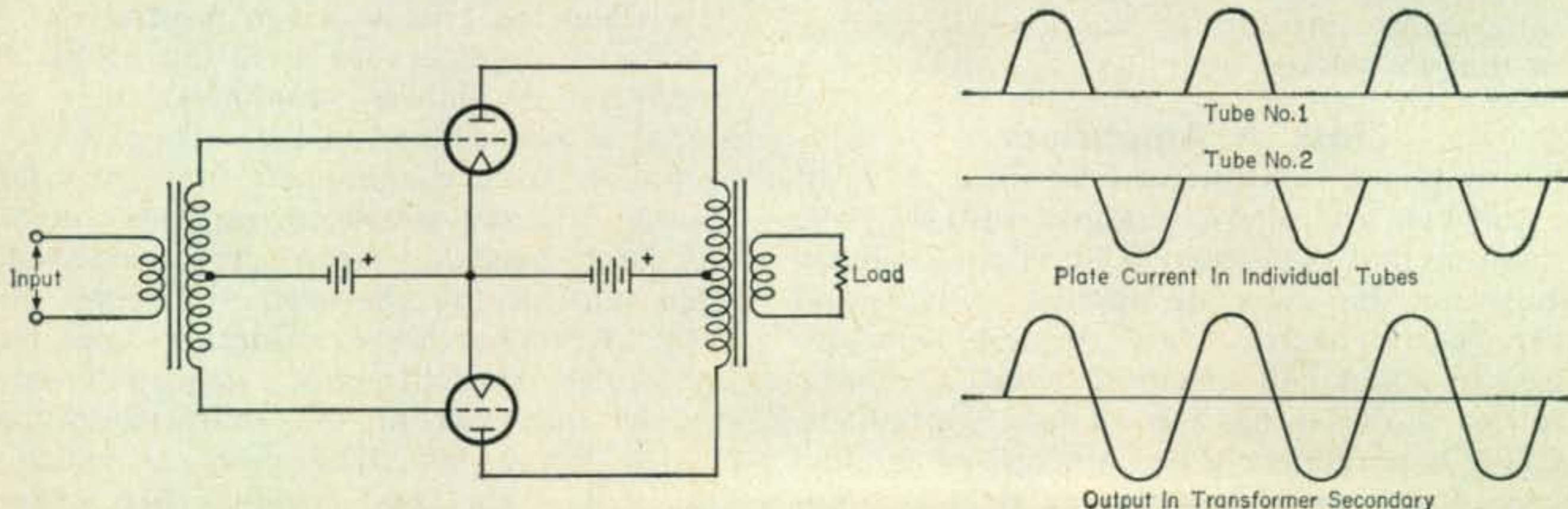
Fig. 3 — It is more common to find two tubes in a Class B r.f. circuit and mandatory in audio applications. In this circuit each tube amplifies alternate half cycles.
