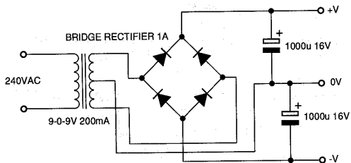
Fig 7. Simple power supply
