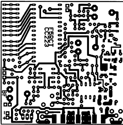
Component side
