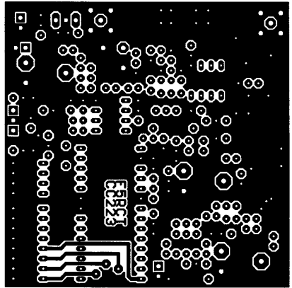
Solder side
