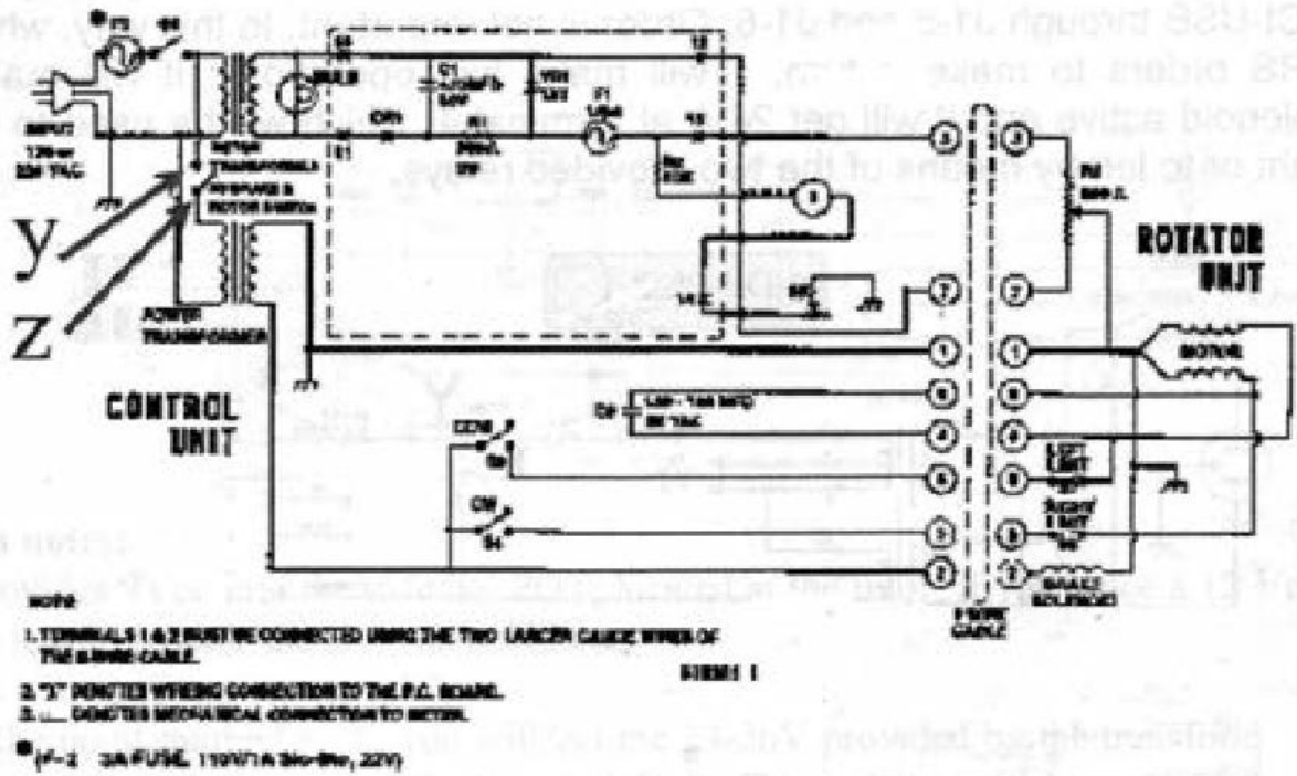
Figure 9 Wiring Schematic
