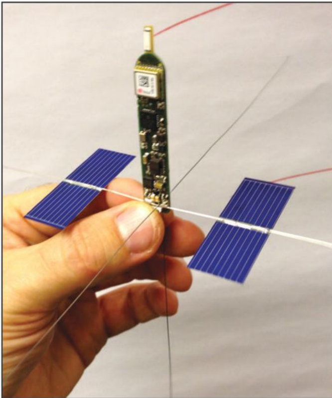
Photo 2. Micro-miniature B-11 transmitter by Leo Bodnar.
