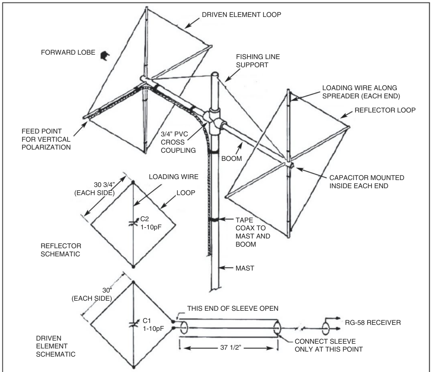
Figure 1. Construction details for the 6-meter shrunken quad. See text for additional information.
