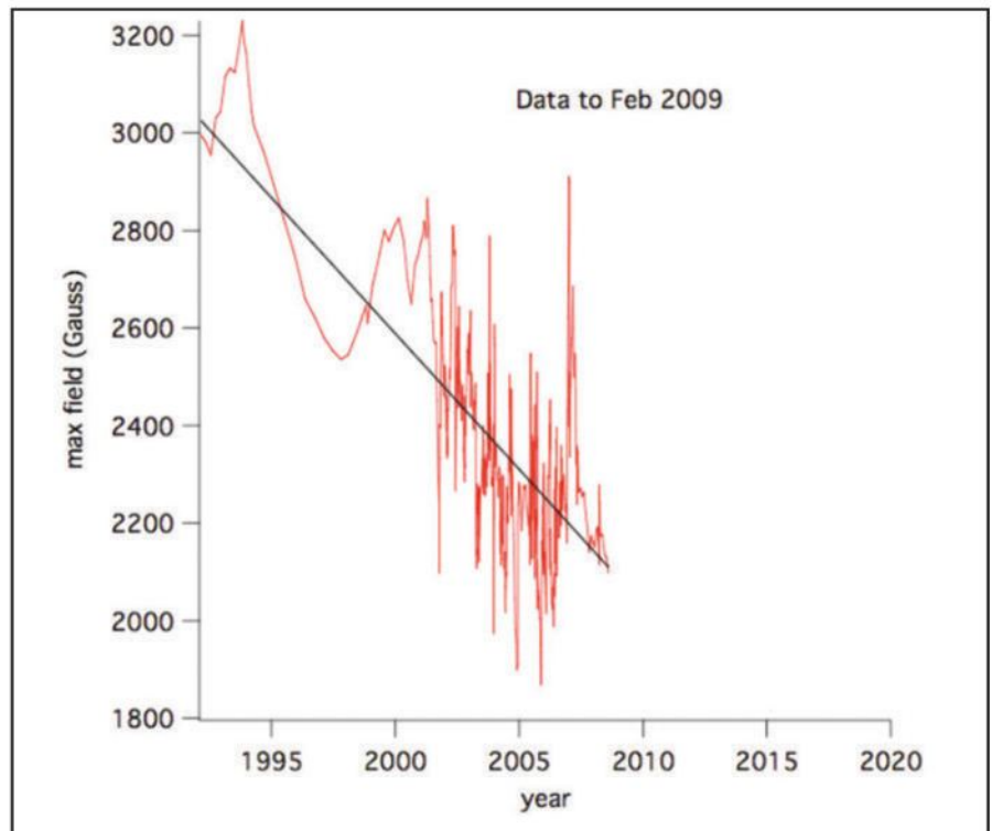
Figure 4. The maximum sunspot field strength is plotted versus time, during the period from 1992 to February 2009; a 12-point running mean is shown, and a linear fit to the data is plotted. Apart from a few measurements, the linear trend has been seen to continue throughout this solar maximum. (Source: M. Penn, U.S. NSO)
