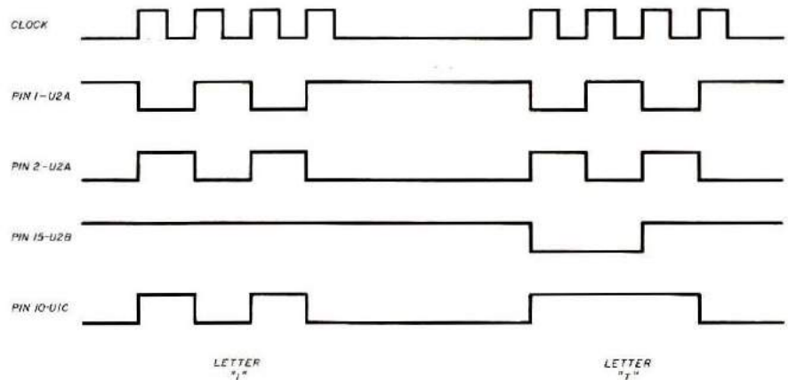
Fig. 2. The train of pulses and logic levels found at various points in the keyer.
