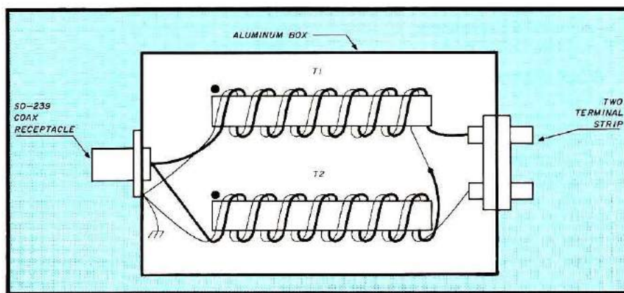
Fig. 4. Transformers T1 and T2 are identical. Each consists of eight bifilar turns of No. 14 (1.6 mm) enamel or Formvar wire. When winding is completed, it will look as if there are sixteen turns in the completed transformer. The wires are wound on side-by-side, the ends being held in a vise to keep tension on as you wind. The ferrite slug is Q-1 material rated for rf application (Indiana-General CF-503). The slug is 12.5 mm (1/2-inch) diameter and about 95 mm (3 3/4 inches) long. The ferrite material is broken to length by nicking it with a file around the circumference, and breaking it with a sharp blow. When completed, the transformer is given a thin coat of Krylon spray. The ends of the winding may be held in place by wrapping the assembly with heavy thread before applying the Krylon. Make sure the windings are interconnected as shown in the diagram, Fig. 3.
