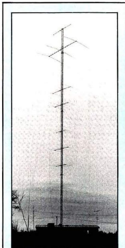
Tired of QRM? Do you ever wonder why some stations seem to work all the DX? This picture of the "antenna tree" at OH8SR (Finland) may provide an insight. The main structure is a rotatable tower 205-foot high, guyed to three slip rings. The tower supports a 40-meter, three-element Yagi on a 40-foot boom at 178 feet elevation; stacked four-element over four-element Yagis for 20 meters at 205 and 141 feet elevations; stacked "four over four" for 15 meters at 121 and 79 feet elevations; and stacked "four over four" for 10 meters at 97 and 64 feet. Listen for the outstanding signal of OH8SR, Markku Nyysönen of Finland, and tell him you saw his antenna photo in Ham Radio Horizons !
