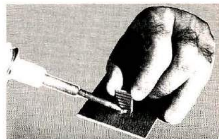
Fig. 2. Now chop the strip down to half-inch pieces, left, and solder the lowest copper pad directly to the baseboard. Use a 35-watt, or larger, soldering iron.
