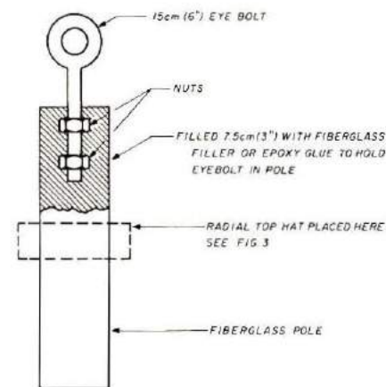
Fig. 2. Mechanical detail of the support screw eye and the method of securing it in the top of the fiberglass pole.
