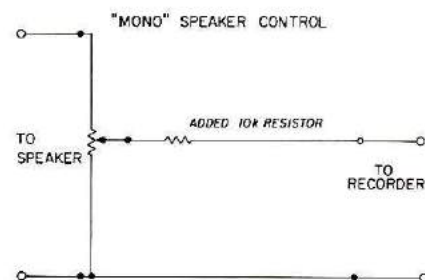
Fig. 1. A "Mono" speaker control can sometimes be used between a loudspeaker and the input to a tape recorder.
