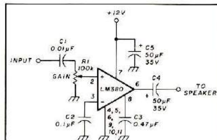
Fig. 6. Simple audio amplifier using the LM380 IC. Circuit provides 1-2 watts of audio power, uses available parts, and can be assembled in a matter of minutes.
