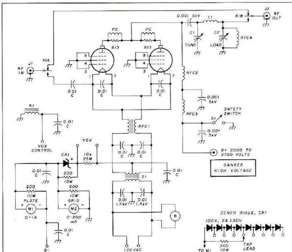
Fig. 1. Schematic diagram for 813 "grounded-grid" linear amplifier.
