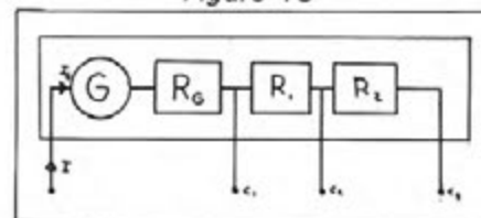
VOLTMETRE Figure 15
