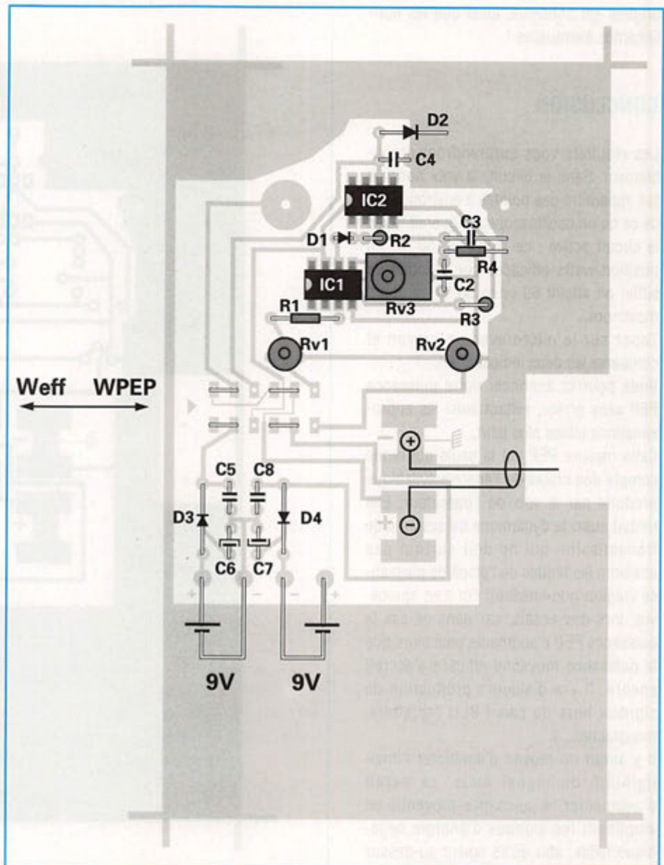
Figure 6 - Implantation des composants.
