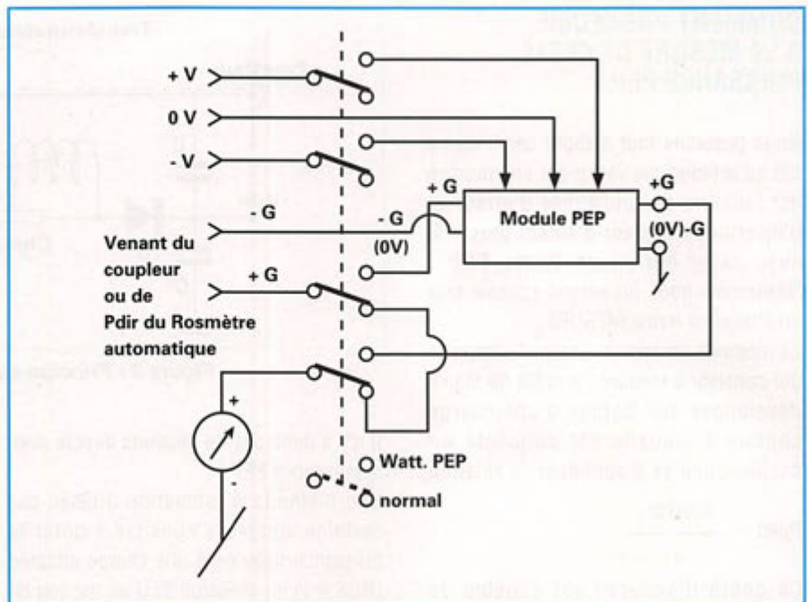
Figure 5 - Interconnexions.
