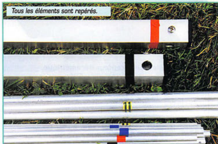
Le gamma-match.
