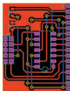
Figure 19: Implantation CI LCD.
