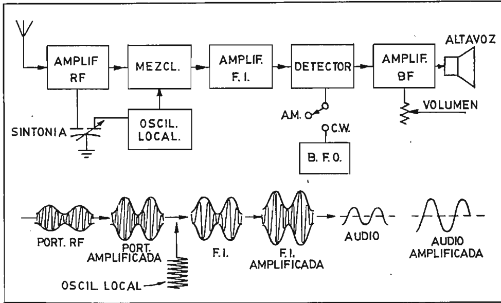
Fig. 55.R - Receptor superheterodino.
