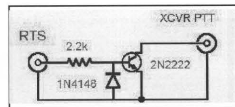
How to connect your PTT to a COM port
