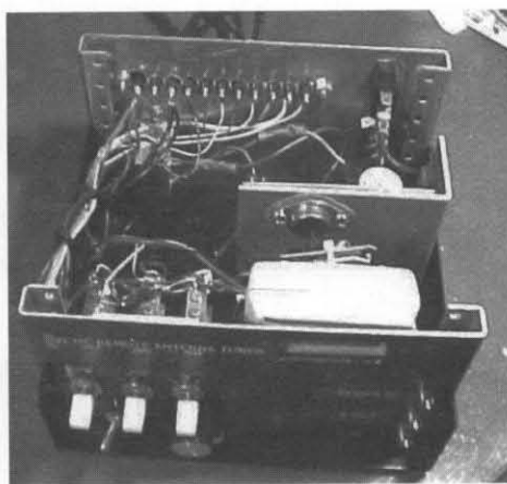
Fig. 2—Internal view of control box.
