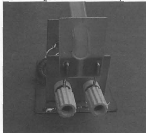
Fig. 1—Front side of twinlead connector, mated to a tuner. The QRP Quarterly
