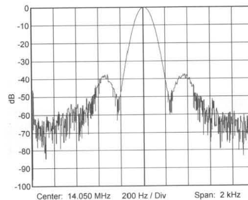
Fig. 3—CW 350 Hz. Sidetone-induced Spurs, 14.050MHz., 5Watt, Ext. Supply
