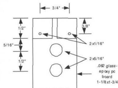
Fig. 3—Connector for small twinlead.
