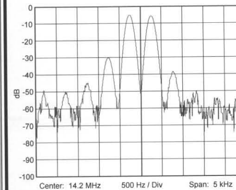
Fig. 7—Two-tone (1000 / 1700 Hz) IMD, 14.200MHz, 2.5 Watts PER, Int.
