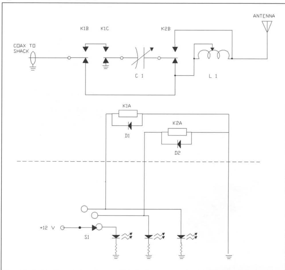
Fig. 3—Motor drive and position indication. Components below the dotted line are located in the control box.
