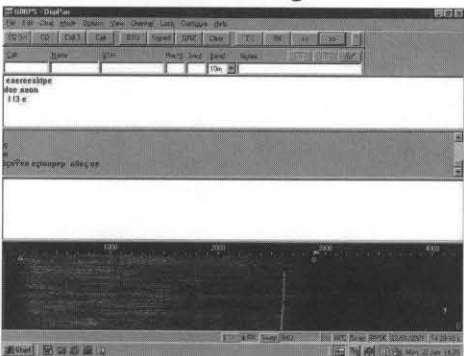
Fig. 3—An SSB voice signal with a CW carrier on the right.
