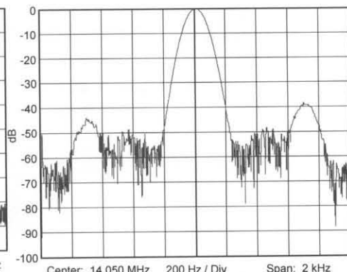
Fig. 4—CW 700 Hz. Sidetone-induced Spurs, 14.050MHz., 5Watt, Ext. Supply
