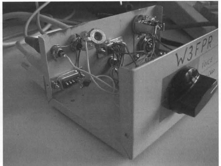
Fig. 3—View of modified switch box.
