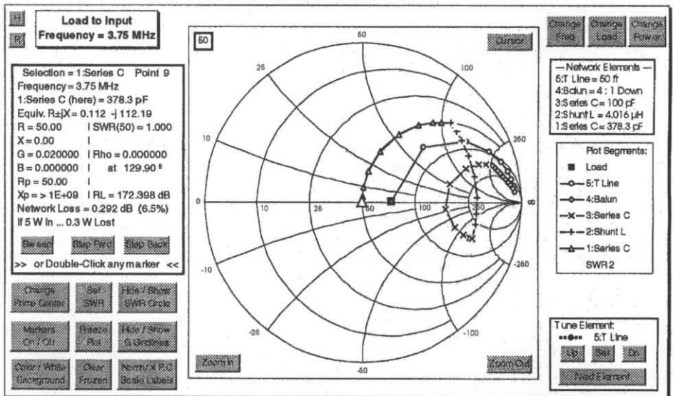
Fig. 2—Impedance transforms continued through the "T" tuner elements. Chart now has a 50 ohm center.
