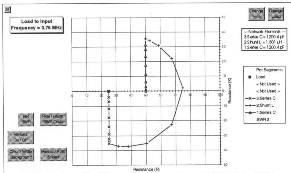
Fig. 6—An alternative way of showing impedance transformations through a "T" tuner. Load is 25+j0 ohms. Elements have no losses in this example.
