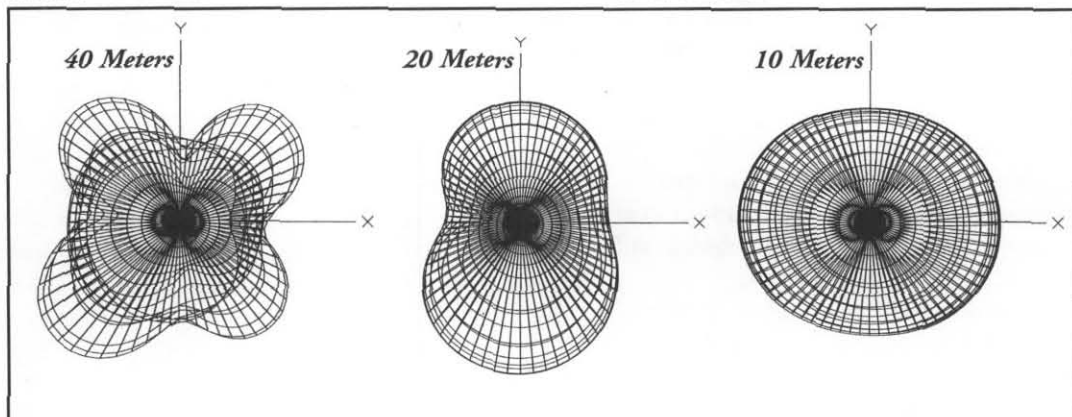
Fig. 3—Examples of EZNEC calculated radiation patterns for OCF End-Fire Array Version 2.
