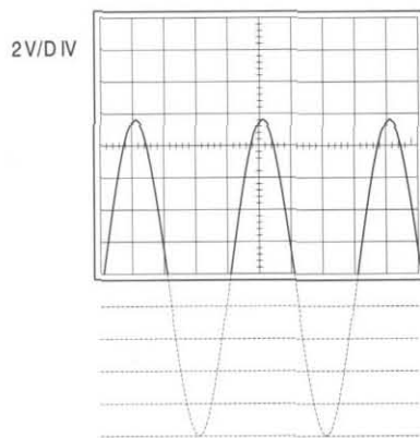
Fig. 12 —Change the sensitivity to 2 volts per division. The peak voltage can be read out from the graticle with better resolution than in figure xx. Double the value to get peak-to-peak voltage.
