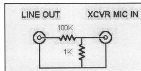
Audio line from the computer to rig
