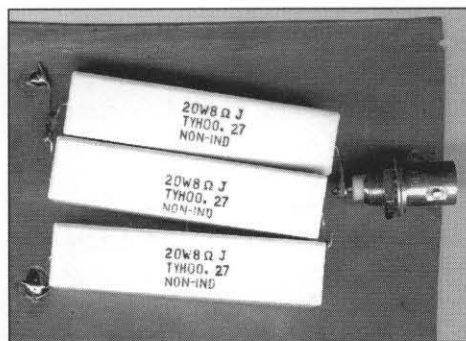
Figure 15—Three 8 ohm “noninductive” resistors in series to ground for the initial network analyzer evaluation. (When this photo was made, the left end of the top resistor was soldered to ground to test a single resistor by itself.)
