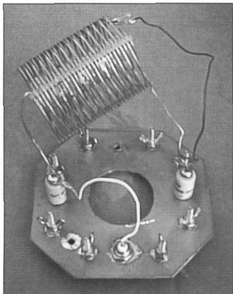
Figure 1—Top view of the base connection plate. The feedline connects from this side.
