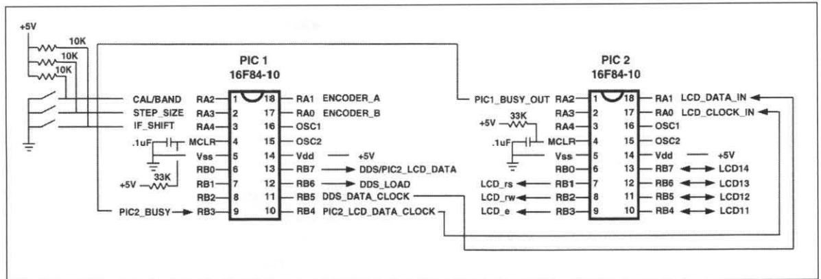
Figure 2. Dual PIC-controlled DDS synthesizer.
