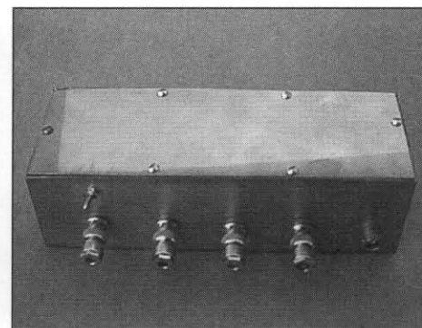
Photo 2. View with covers installed.
