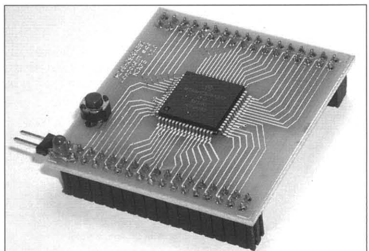
Figure 5. HC908 Daughtercard.
