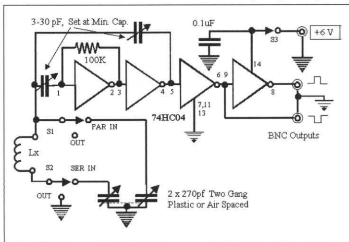
Figure 1. The circuit.
