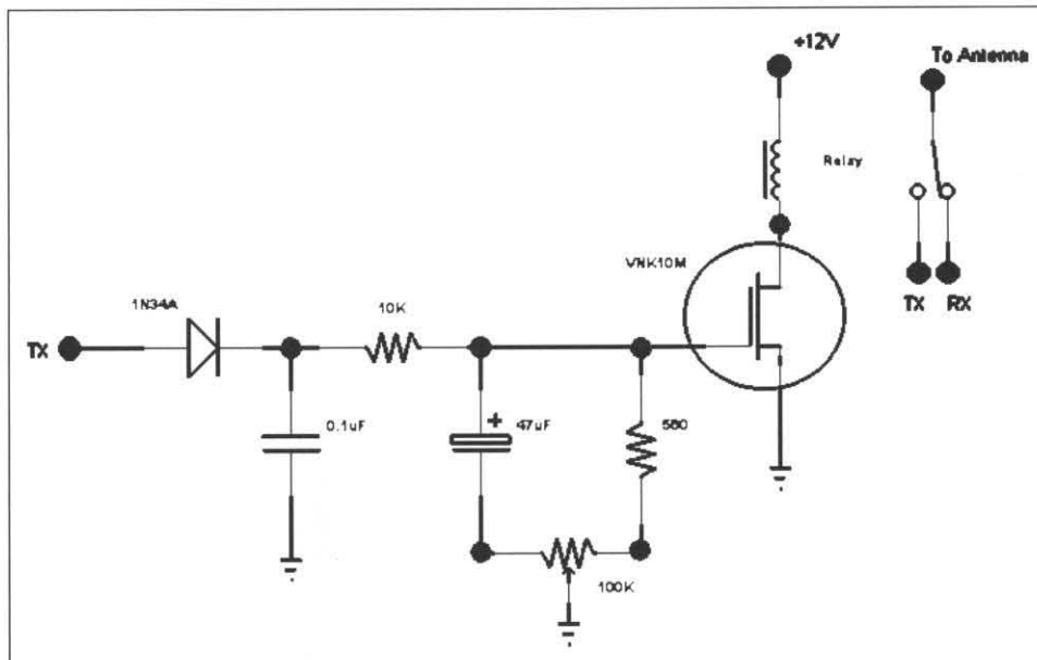
RF Sensing Transmit/Receive Switch
