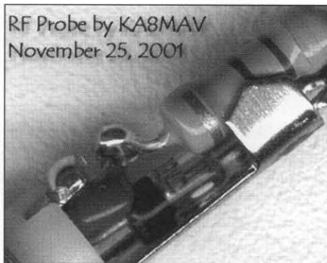
Figure 14—Another close-up of the components. The diode is more visible in this photo than the last.
