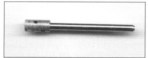
Figure 7—The "Islander" pad cutter from NJQRP, a diamond tipped tool for making "street level" pads for Manhattan construction.
