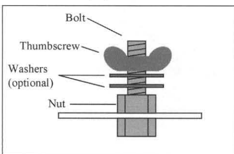
Figure 5—Use nuts, bolts, thumbscrews (and optional washers) to connect bare wires to the base plate [WA8MCQ drawing].
