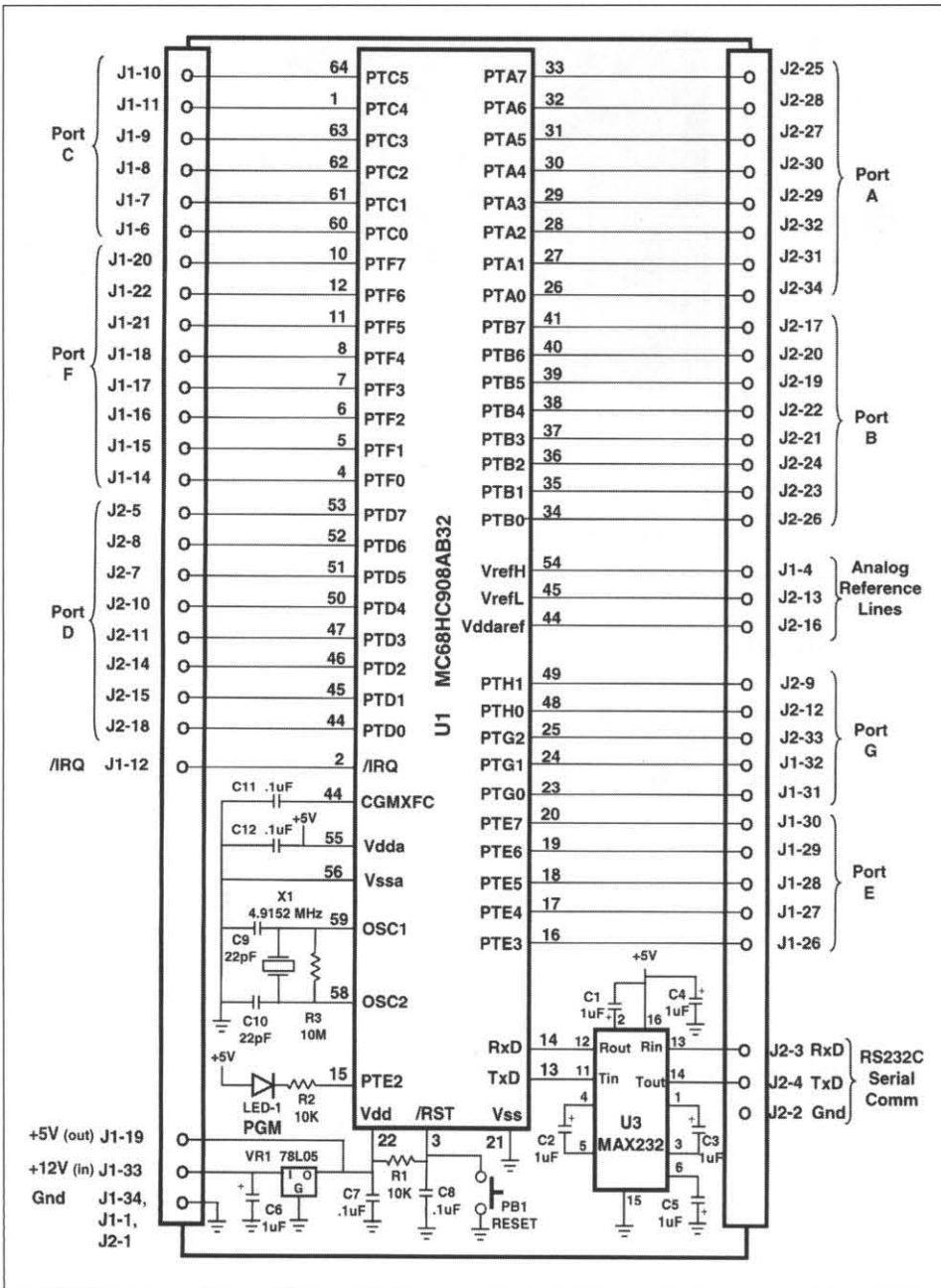
Figure 7. Schematic for the Digital QRP BreadBoard system—Phase 1.
