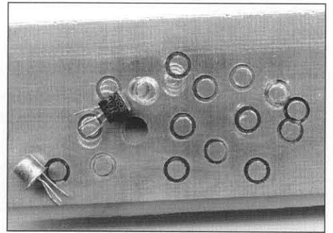
Figure 8—Some test pads made with the cutter, with a pair of transistors for reference. (Some of the rings are darker than others; I was having a hard time getting a satisfactory picture and was experimenting with darkening some rings with a marker for better contrast.)
