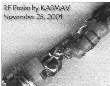
Figure 13—Close-up of the components.
