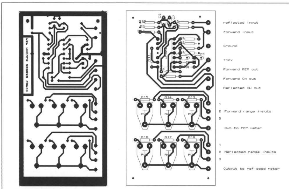
PCB foil pattern (left) and parts layout of the CW/PEP conversion board.
