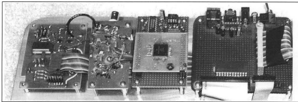
Figure 6—Photo showing layout of the project during heavy-duty debug.
