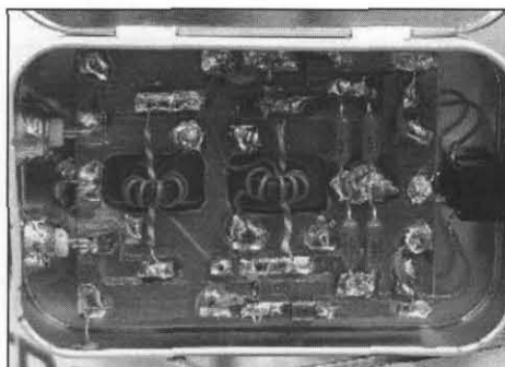
W3IRZ's original NoGaWatt prototype, inside and outside. Photos courtesy of the North Georgia QRP Club.
