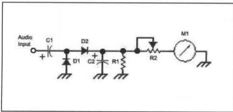
A simple signal-strength measuring circuit (diode detector).
