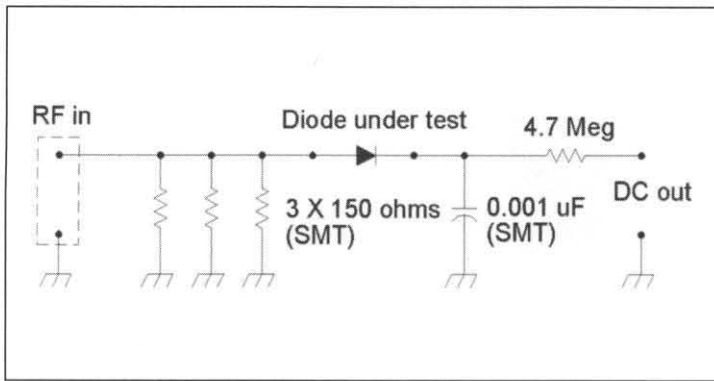
Figure 19 —Schematic of the diode test fixture. By the time I was done, I had 18 identical circuits built with surface mount parts on 2 pieces of scrap PCB stock. The PCB pads were milled out and are identical at all 18 positions.
