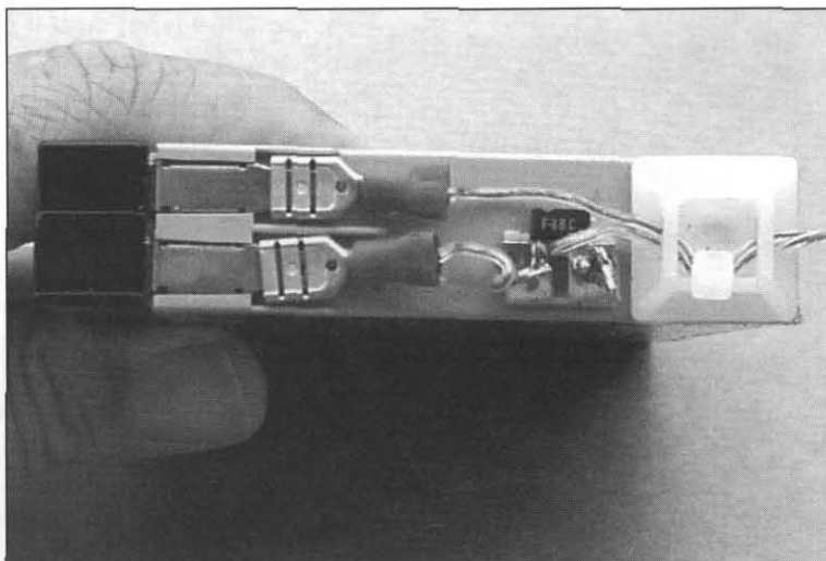
Figure 4—Top of battery with quick-disconnect connectors and solid-state fuse mounted on piece of PCB material.
