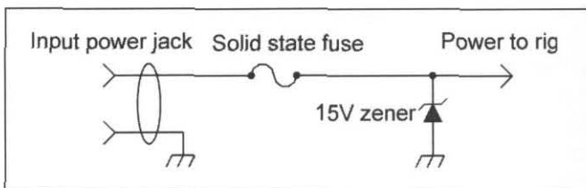
Figure 3—Modernized “dummy diode” with solid-state “fuse.”
