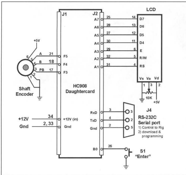
Figure 11—Schematic. Simple I/O devices (shaft encoder, LCD, serial port and a pushbutton) are all that's needed to allow the HC908 Daughtercard to perform as a CI-V intelligent serial controller for your rig.
