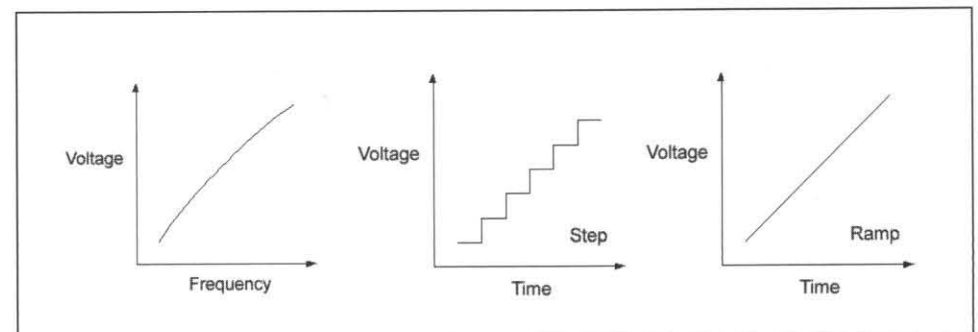
The voltage-to-frequency characteristic (left) of the VCO can be controlled by either a series of voltage steps (center) or a continuous voltage ramp (right).
