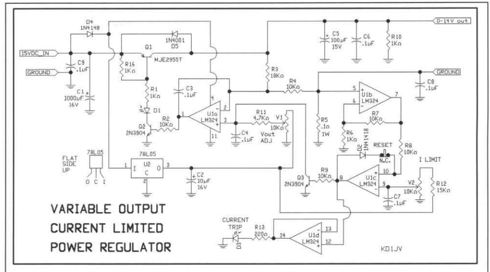
Figure 1. Schematic diagram of the regulated power supply.
