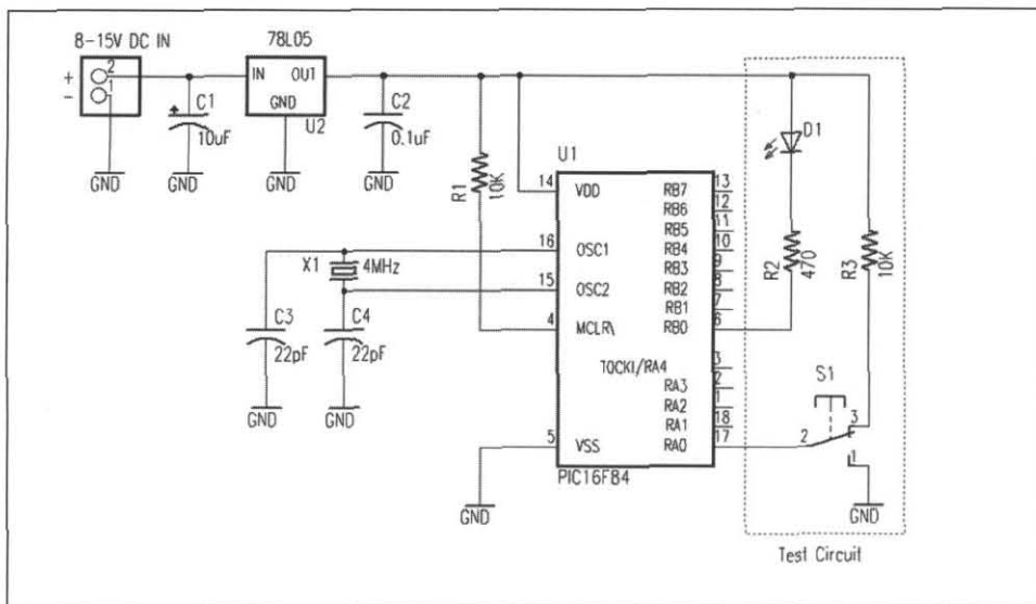
Figure 2—Diagram of the PIC demonstration circuit.
