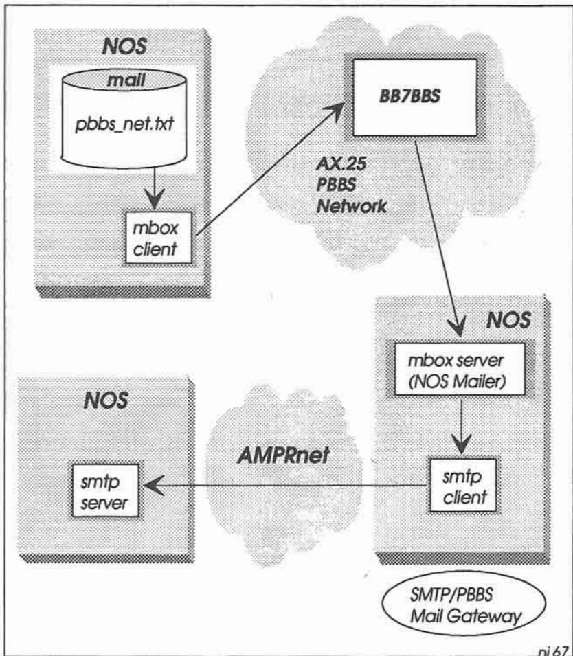
Fig 25-1: Forwarding mail to a NOS station via the PBBS network. The mailbox client forwards .txt files in the mail queue (/spool/mail) to a neighbouring AX.25 PBBS (BB7BBS). This BBS then forwards the mail to an SMTP/PBBS mail gateway. The gateway converts the mail to SMTP format, and forwards it via AMPRnet to the final destination.
